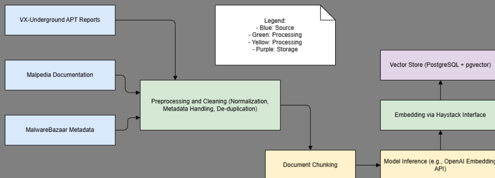
FIGURE 3.2: RAG Corpus Construction Pipeline
