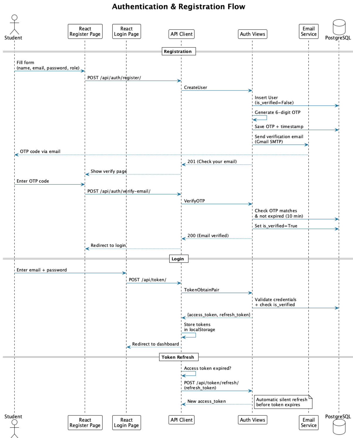
Figure 4: Authentication and Registration Flow
