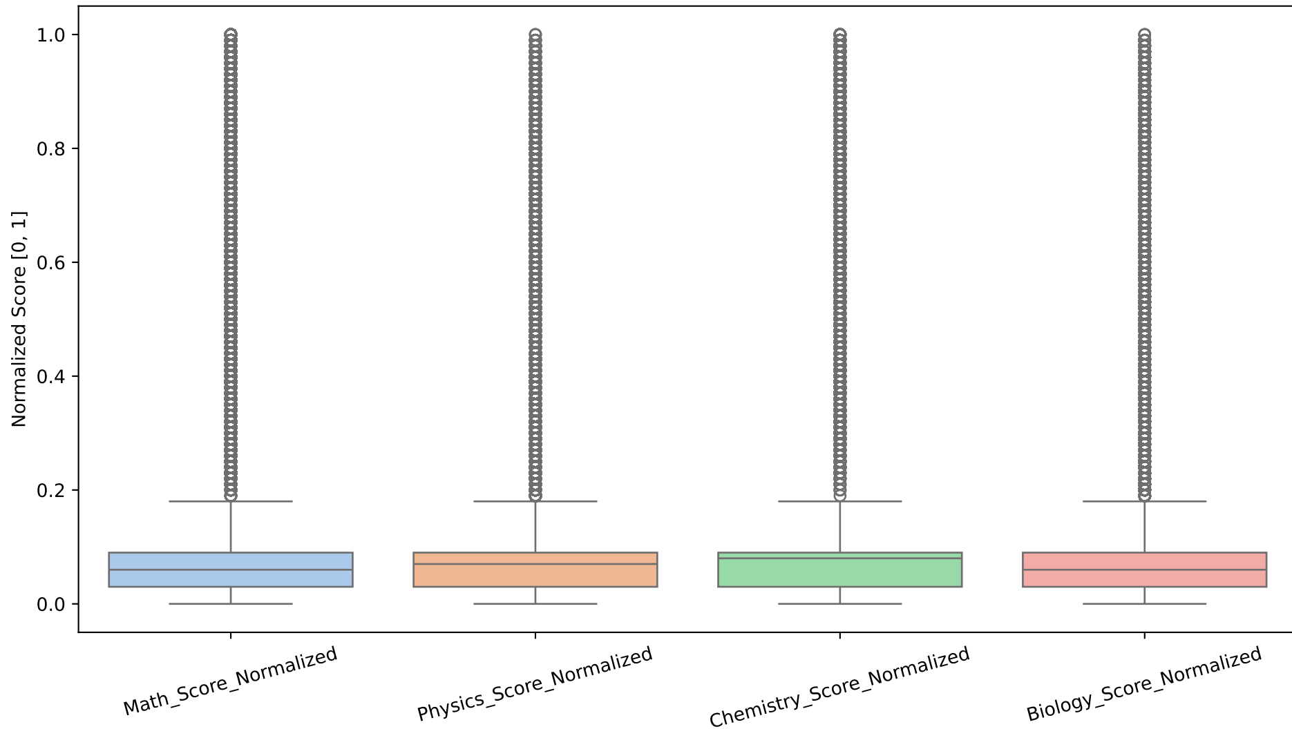
Distribution of Normalized STEM Scores
