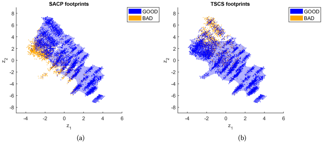
Fig. 8. Footprints for SACP (a) and TSCS (b), where good performance means relatively best (minimal constraint violations) compared to the other algorithm. Ties were not broken.
