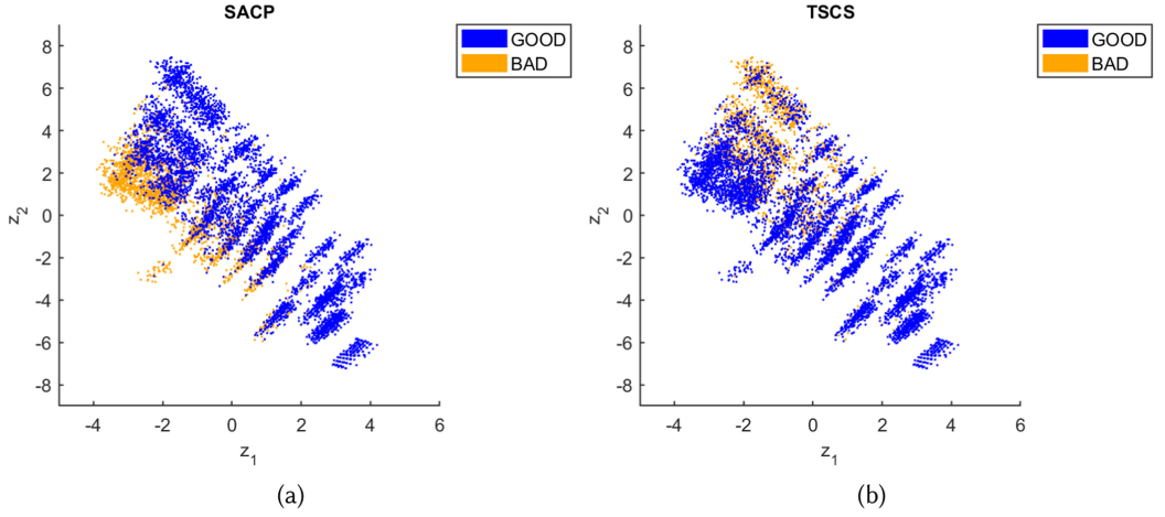
Fig. 6. Instances where each algorithm achieves the best performance in blue (minimal constraint violations) for SACP (a) and TSCS (b), without breaking ties. Orange shows instances where the best performance was not obtained by each algorithm.
