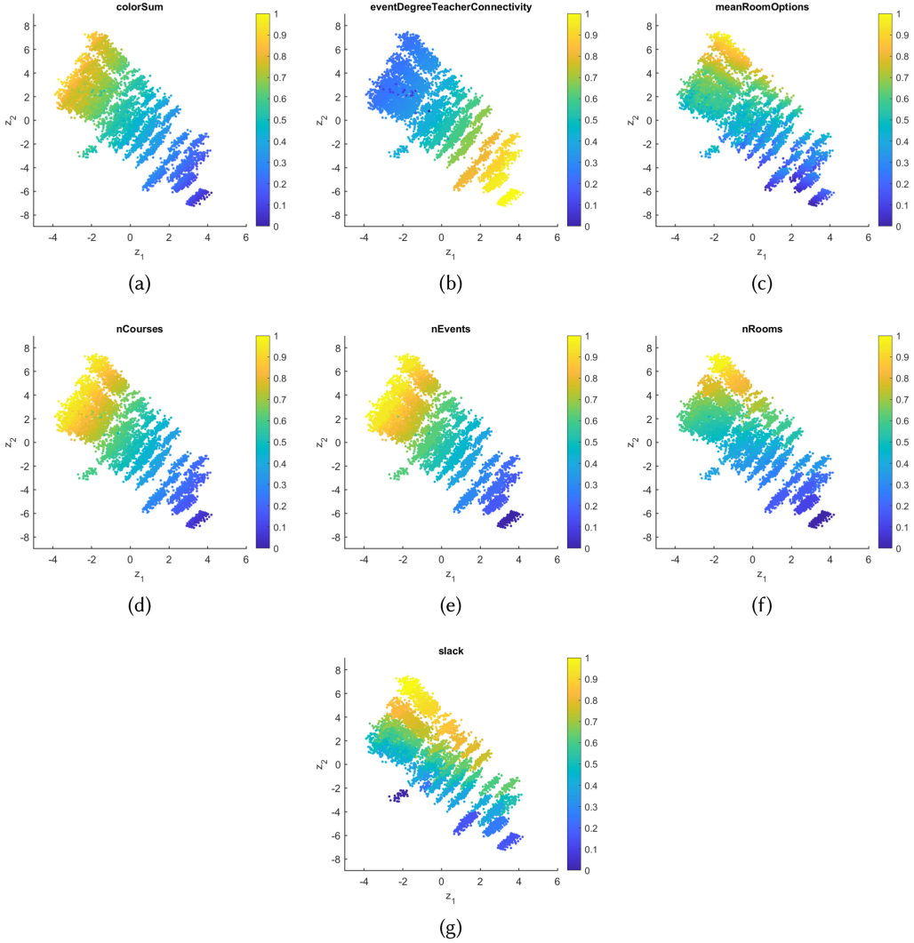
Fig. 10. Feature distributions for colorSum (a), eventDegreeTeacherConnectivity (b), meanRoomOptions (c), nCourses (d), nEvents (e), nRooms (f), and slack (g). Minimal values of each feature are indicated by coloring an instance blue and maximal feature values shown as yellow.
