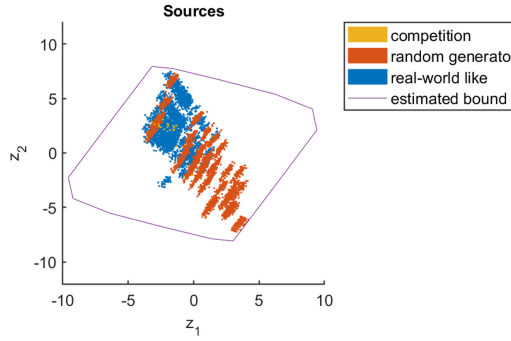
Fig. 3. Timetabling instance space defined by Equation (10) showing three sources of instances, and estimated boundary of instance space.
