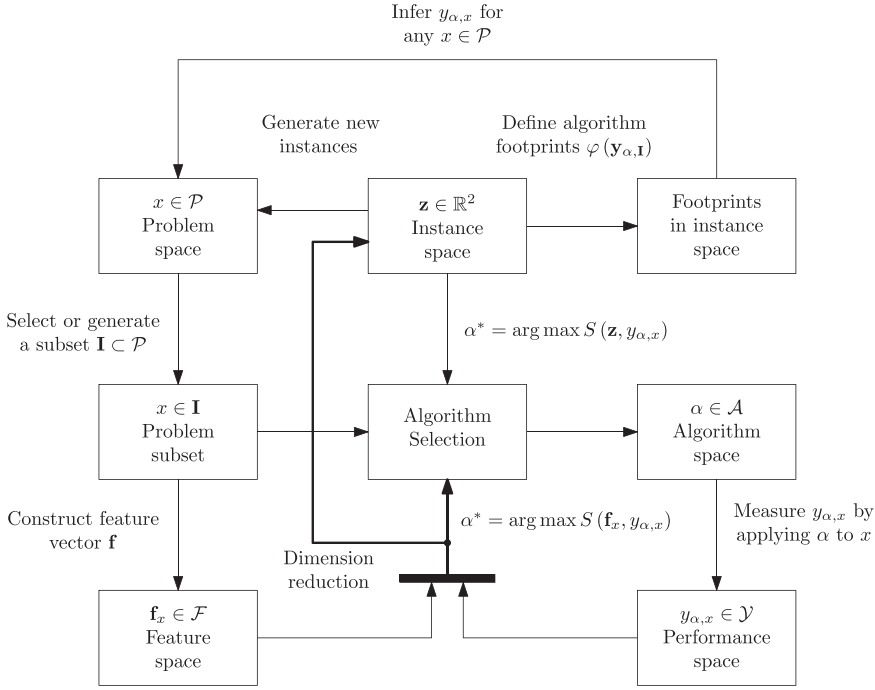
Fig. 1. Summary of the ISA framework.
