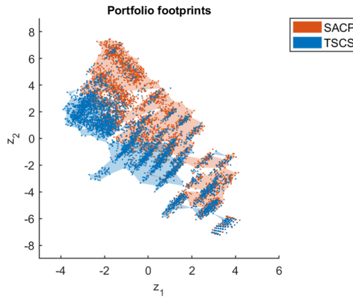
Fig. 9. Footprints where each portfolio is best (based on actual performance). Ties were broken randomly. Overlapping areas indicate that purity is the same for both algorithms, hence not enough evidence exists that one of them dominates.
