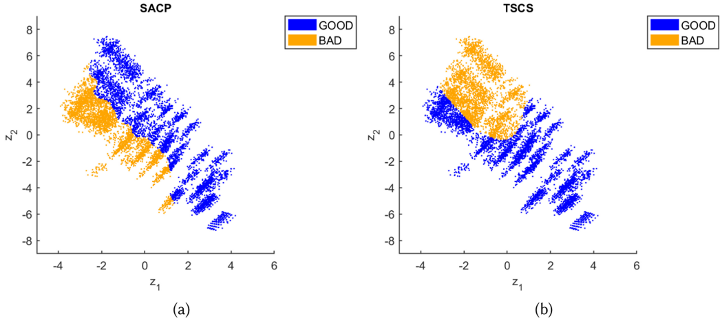
Fig. 4. SVM predicted performance of SACP (a) and TSCS (b), where good performance means relatively best (minimal constraint violations) compared to the other algorithm.
