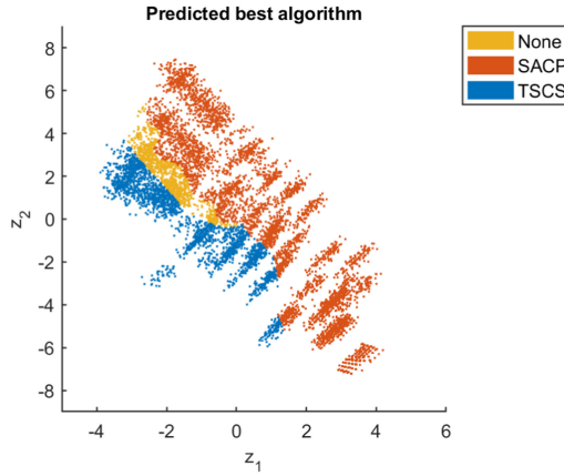
Fig. 5. Recommended algorithms from SVM prediction models, including the region where neither algorithm has sufficient evidence for recommendation as best.
