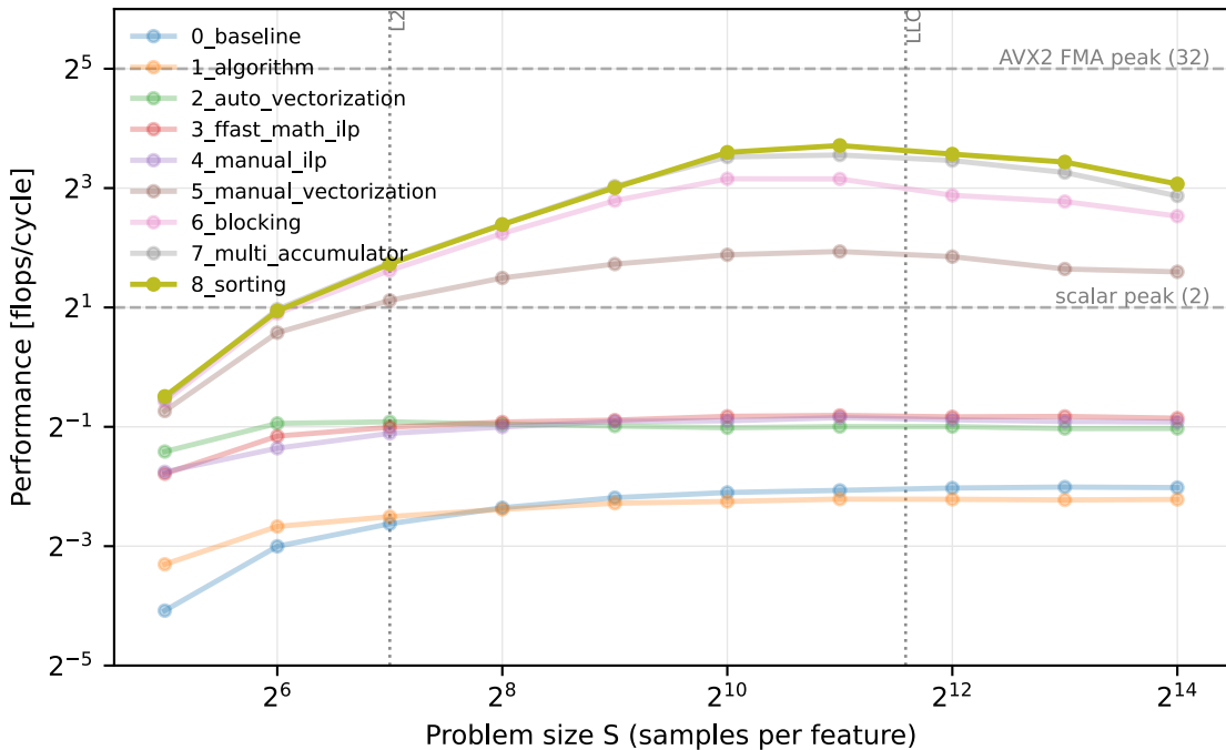
Performance Scaling (Up to 8_sorting)
