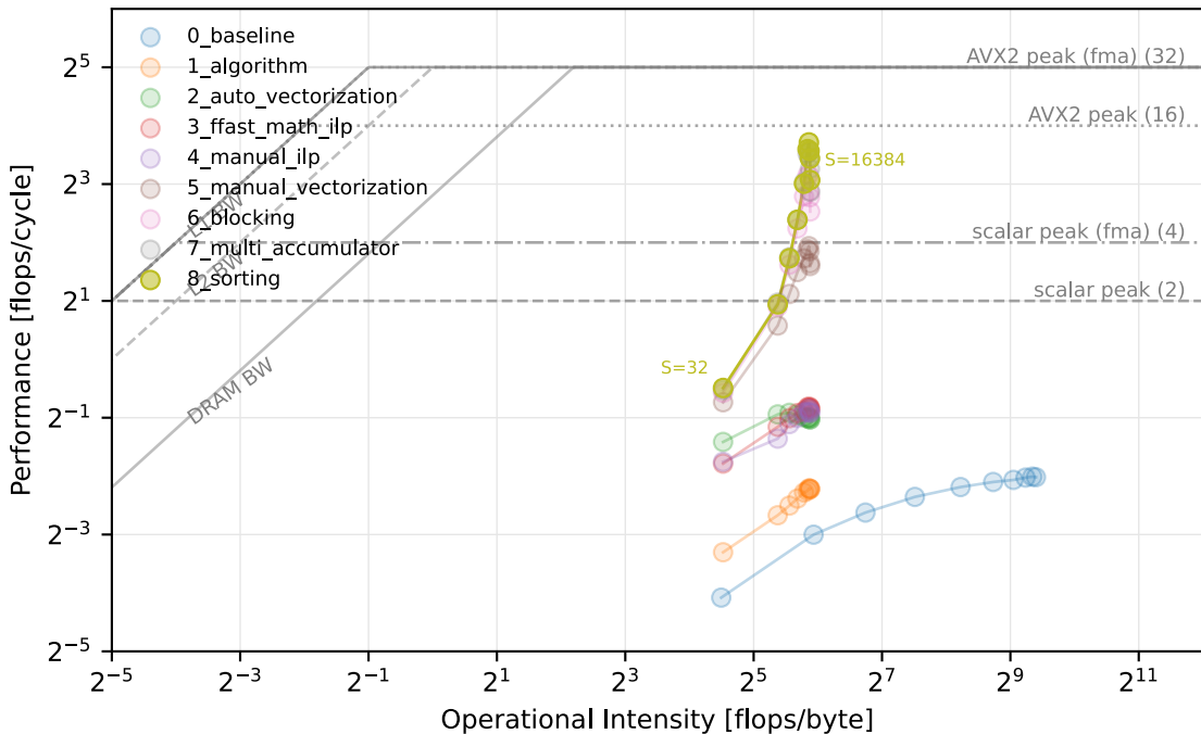
Roofline (Up to 8_sorting)
