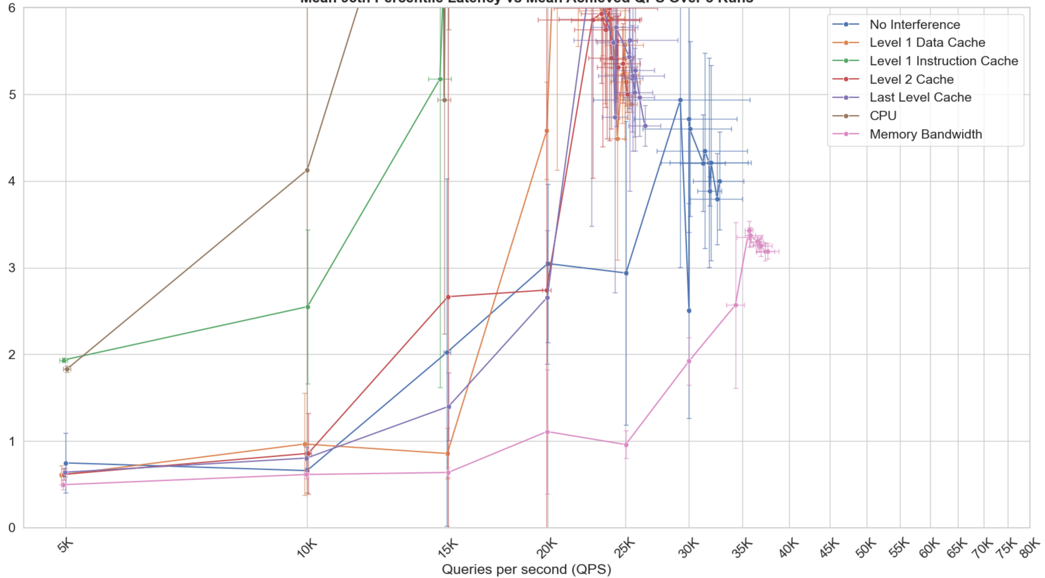
Mean 95th Percentile Latency vs Mean Achieved QPS Over 3 Runs
