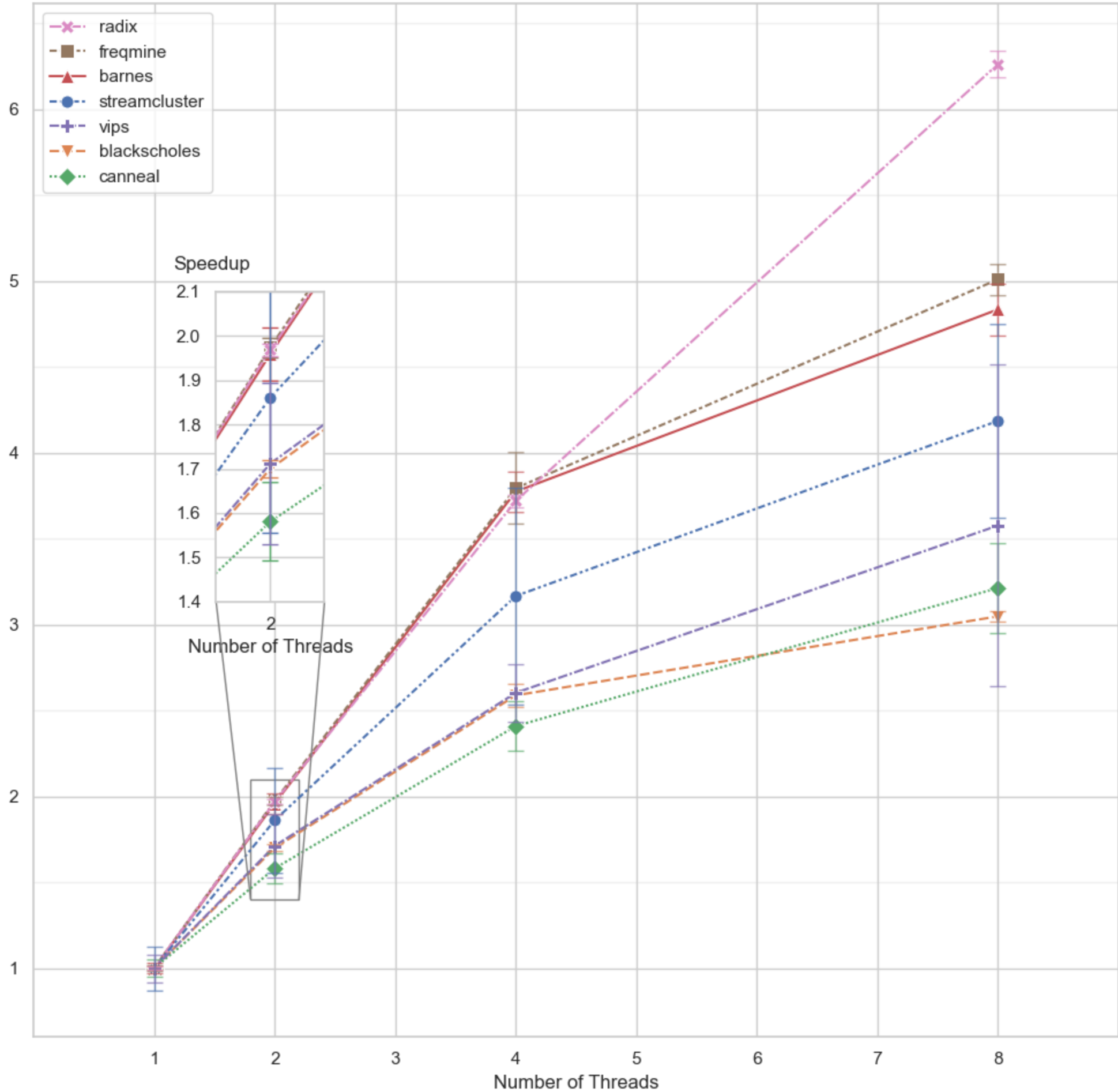
Speedup of the Benchmark compared to the number of Threads
