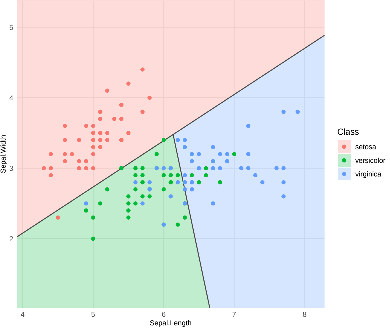
Decision Boundaries
