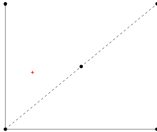
(f) RecLMTD - (4, 3, 1)
