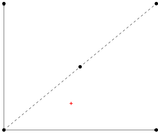
(c) RecLMTD - (2, 1, 1)
