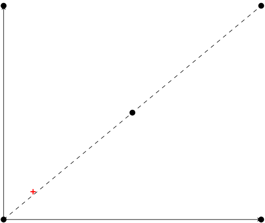
(g) RecLMTD - (5, 4, 1)
