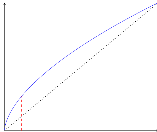
(f) q^\beta - (4, 3, 1)
