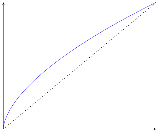
(c) q^\beta - (2, 1, 1)
