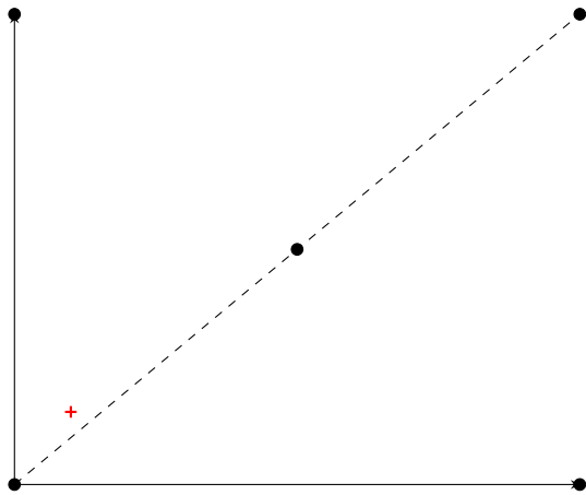
(e) RecLMTD - (3, 5, 1)
