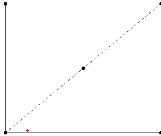
(b) RecLMTD - (1, 4, 2)
