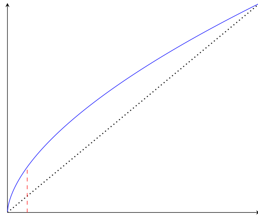
(b) q^\beta - (1, 4, 2)
