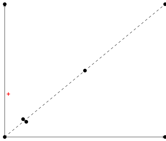
(g) RecLMTD - (5, 4, 2)
