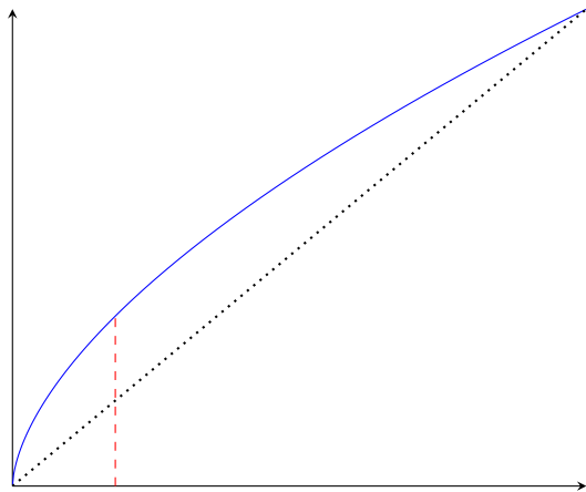
(a) q^\beta - (1, 3, 2)
