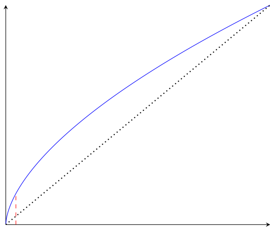
(c) q^\beta - (2, 3, 1)
