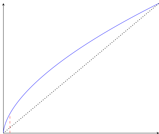
(e) q^\beta - (4, 2, 1)
