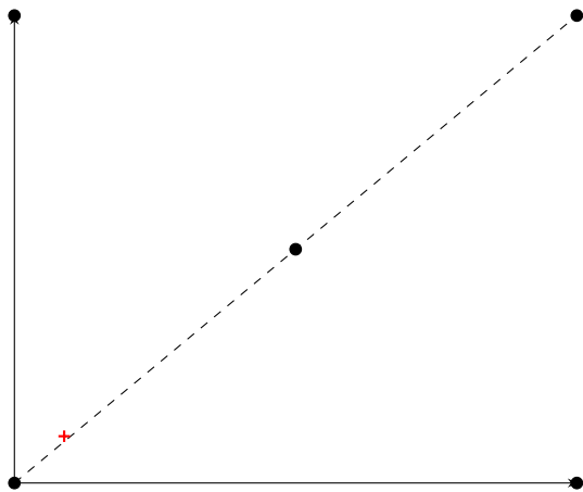
(c) RecLMTD - (2, 3, 1)
