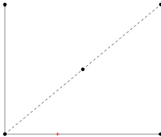
(f) RecLMTD - (4, 5, 1)
