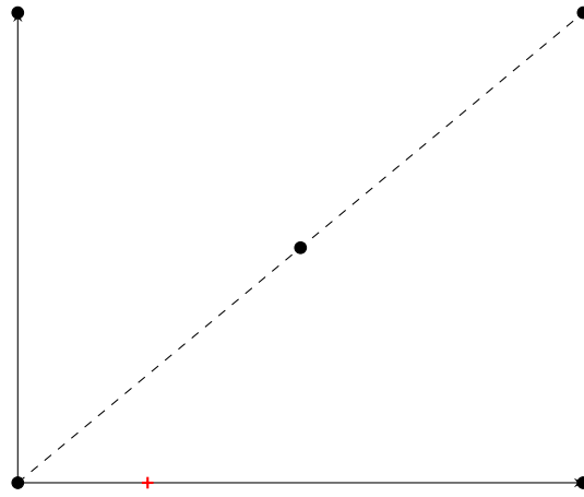
(h) RecLMTD - (5, 5, 2)
