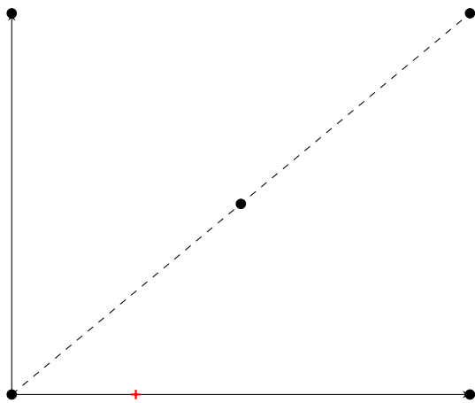
(e) RecLMTD - (4, 2, 1)
