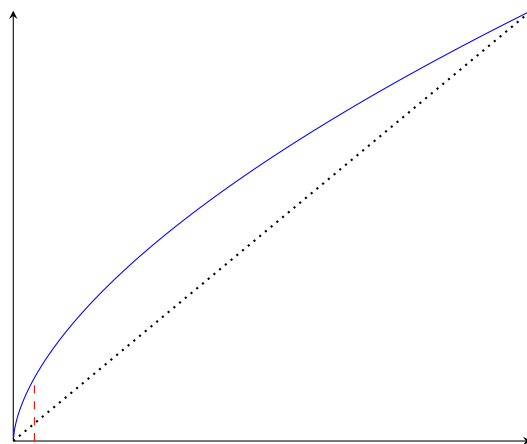
(f) q^\beta - (4, 5, 1)
