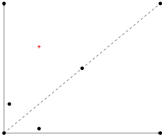
(g) RecLMTD - (5, 1, 1)
