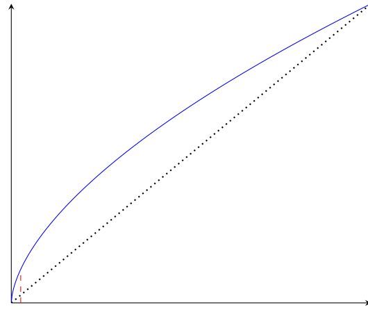
(h) q^\beta - (5, 5, 2)
