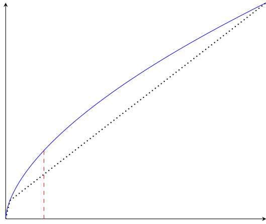
(g) q^\beta - (5, 1, 1)
