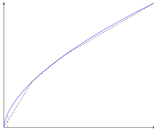
(b) q^\beta - (2, 2, 1)
