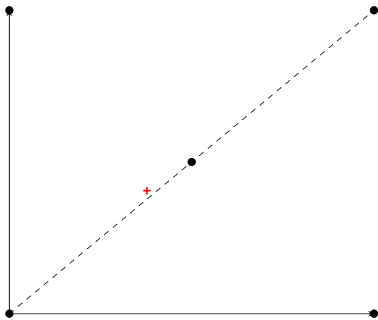
(a) RecLMTD - (1, 3, 2)
