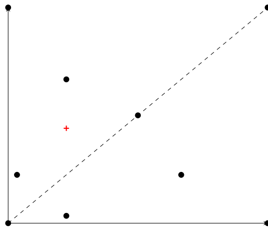
(f) RecLMTD - (5, 1, 1)
