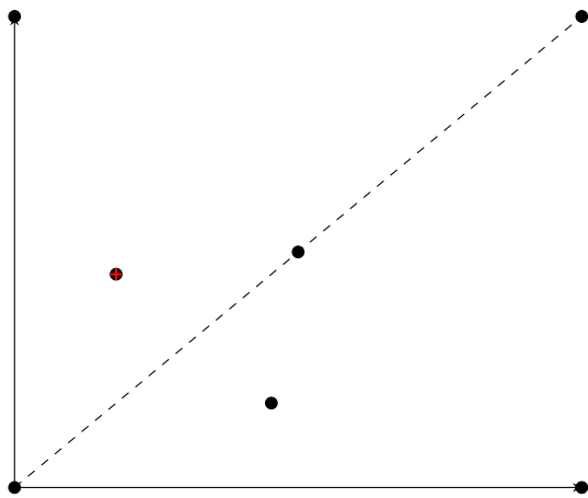
(e) RecLMTD - (4, 3, 1)
