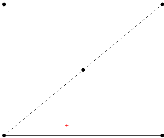
(c) RecLMTD - (2, 4, 1)
