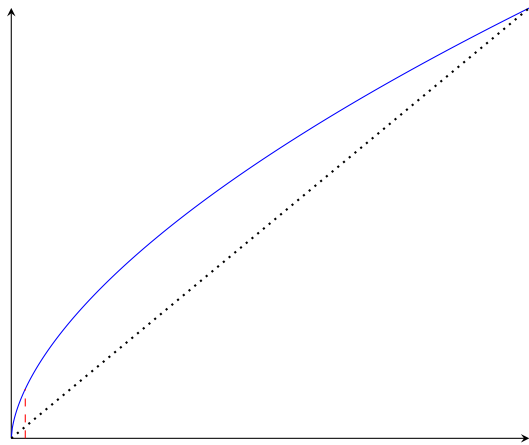
(c) q^\beta - (2, 4, 1)
