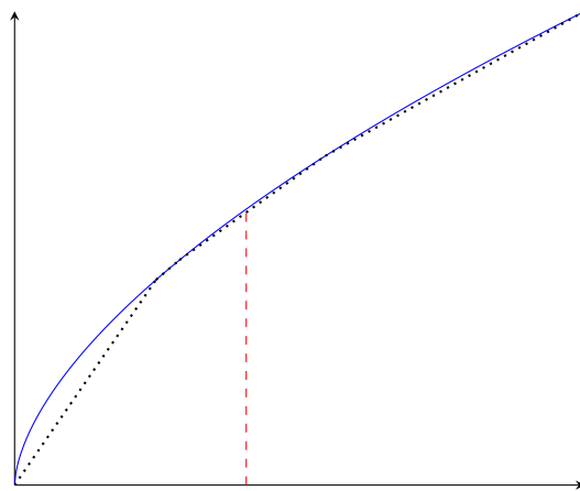
(b) q^\beta - (2, 2, 2)
