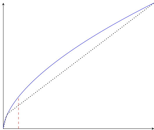
(c) q^\beta - (2, 5, 2)
