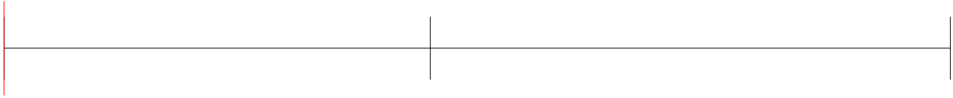
(a) t^{(H)} - (2, 2, 2)
