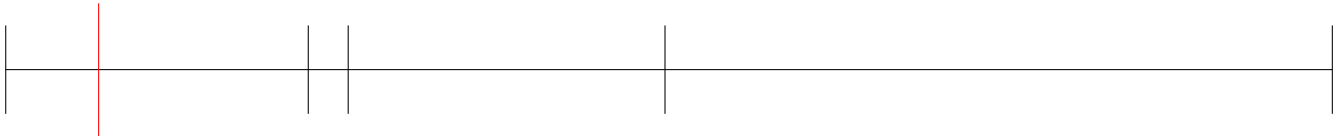
(a) t^{(H)} - (5, 4, 2)
