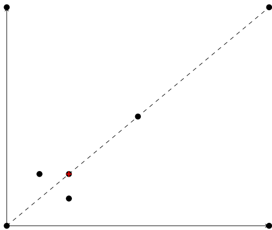
(c) RecLMTD - (2, 5, 2)
