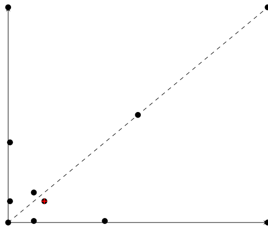
(b) RecLMTD - (2, 2, 2)
