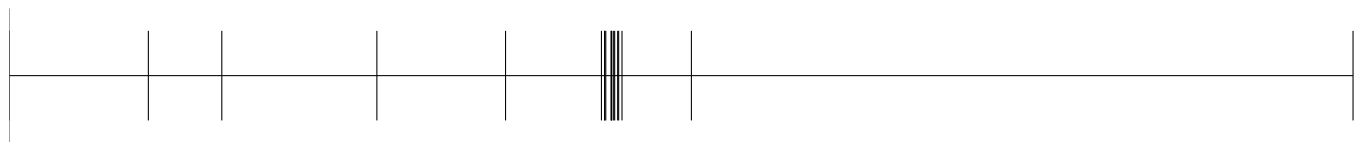
(a) t^{(H)} - (2, 1, 2)
