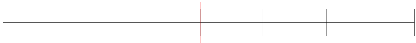
(a) t^{(H)} - (1, 1, 1)
