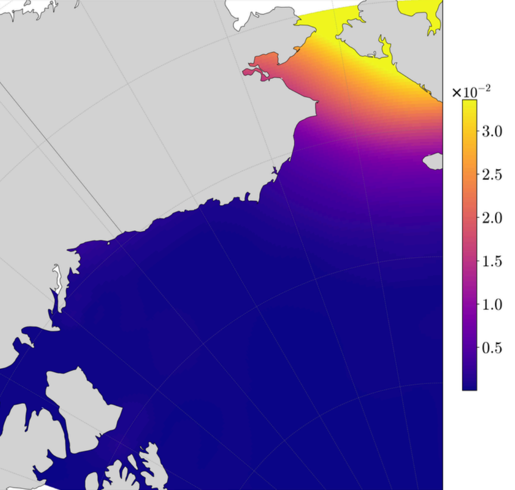
Copernicus AMJ Satellite SLA Std Dev (m)
