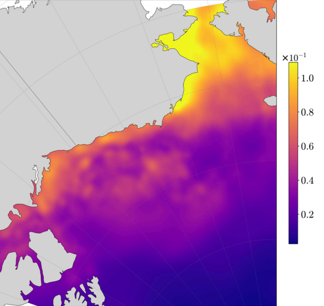
Copernicus 1999 Satellite SLA Std Dev (m)
