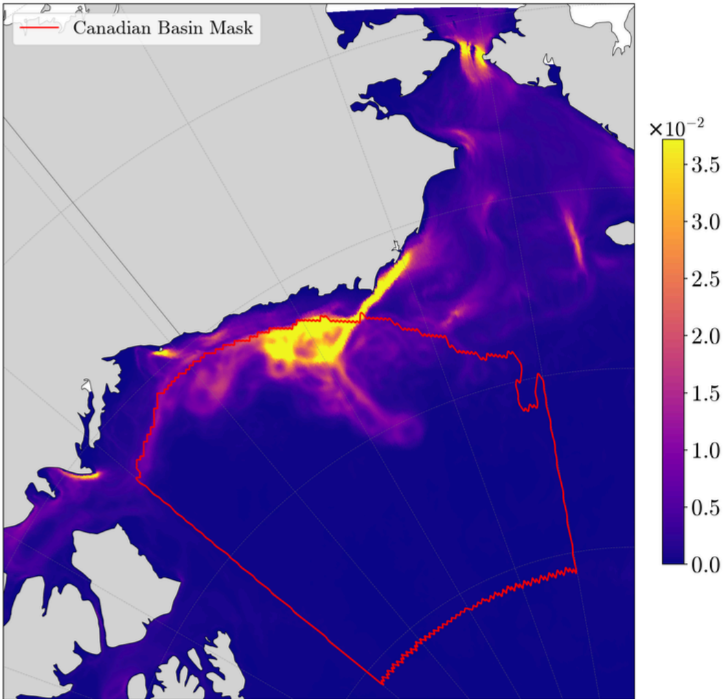
ARC60 1995 Average Eddy Kinetic Energy From 0 to 50 m Depth ( \text{m}^2/\text{s}^2 )
