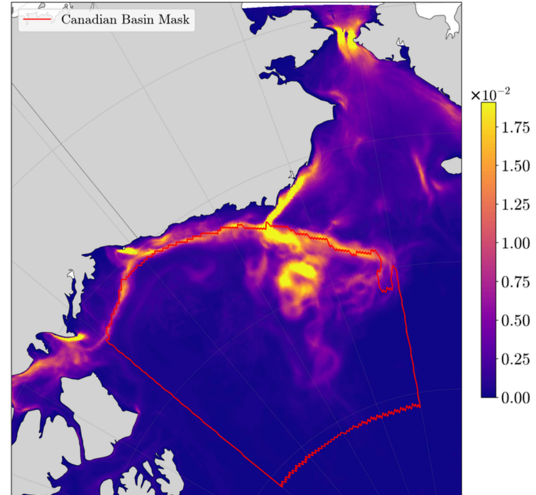
ARC60 1999 Average Eddy Kinetic Energy From 0 to 50 m Depth ( \text{m}^2/\text{s}^2 )
