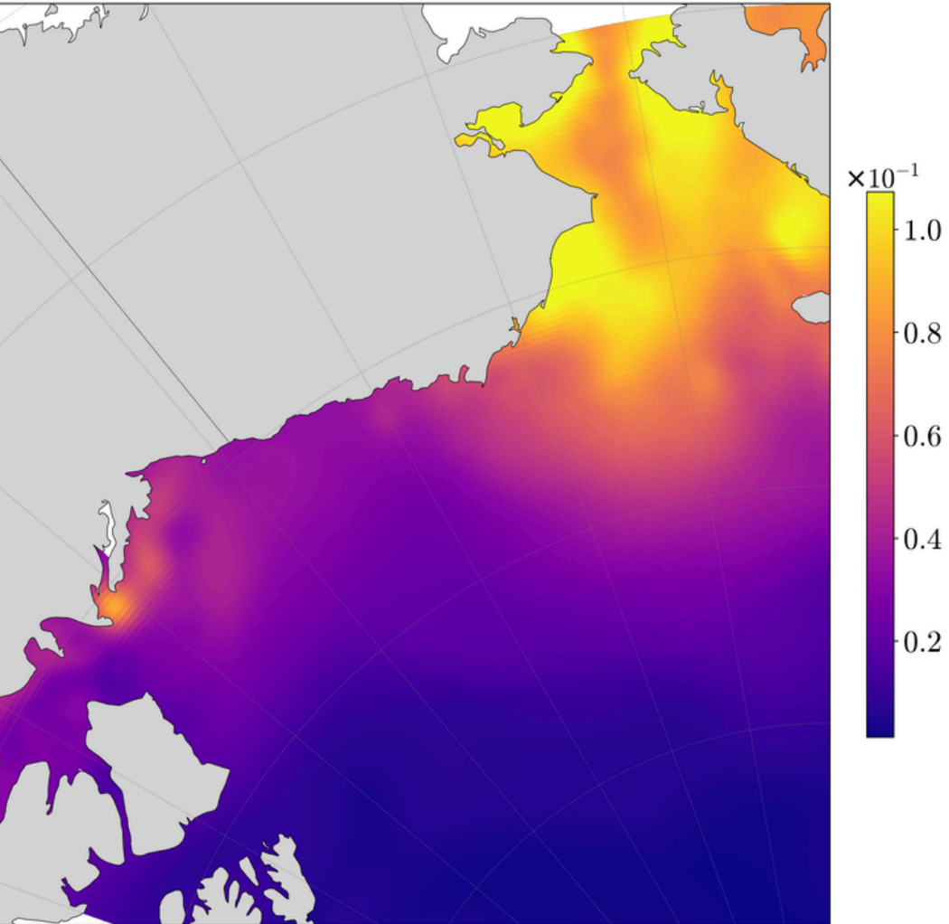
Copernicus 1997 Satellite SLA Std Dev (m)
