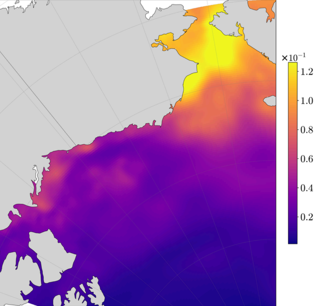
Copernicus 1995 Satellite SLA Std Dev (m)
