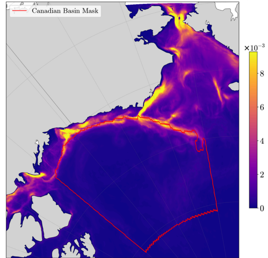
ARC60 1999 Average Eddy Kinetic Energy From 0 to 50 m Depth ( \text{m}^2/\text{s}^2 )
