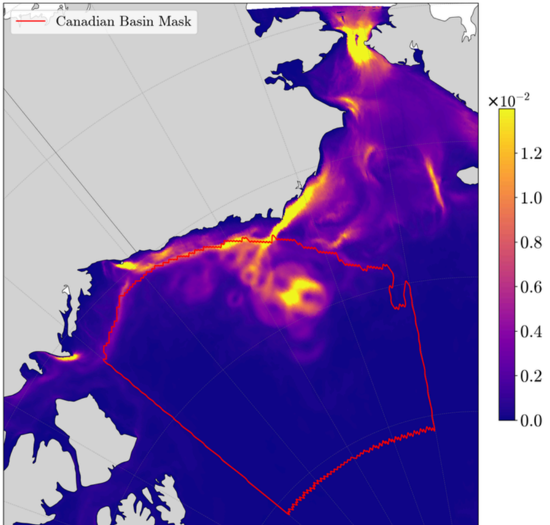
ARC60 AMJ Average Eddy Kinetic Energy From 0 to 50 m Depth ( \text{m}^2/\text{s}^2 )
