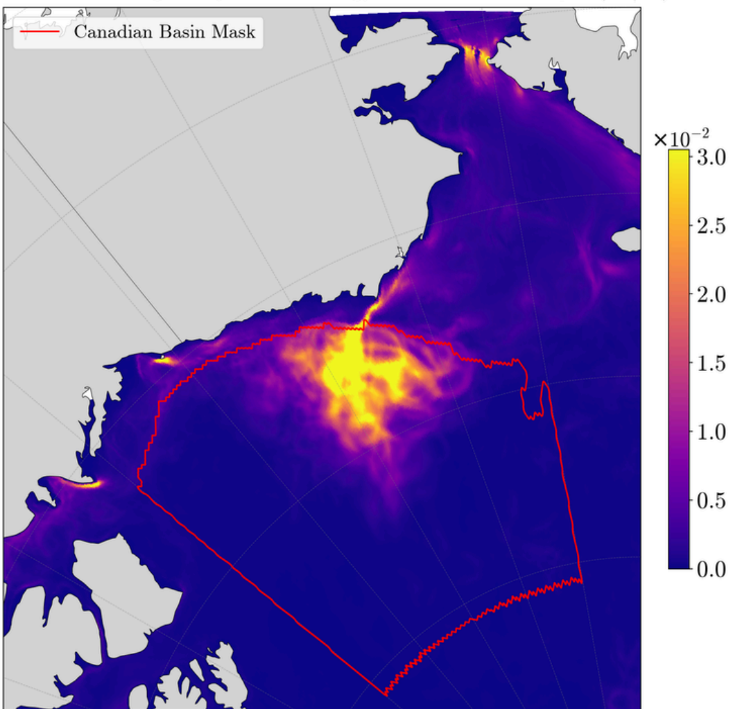
ARC60 1997 Average Eddy Kinetic Energy From 0 to 50 m Depth ( \text{m}^2/\text{s}^2 )
