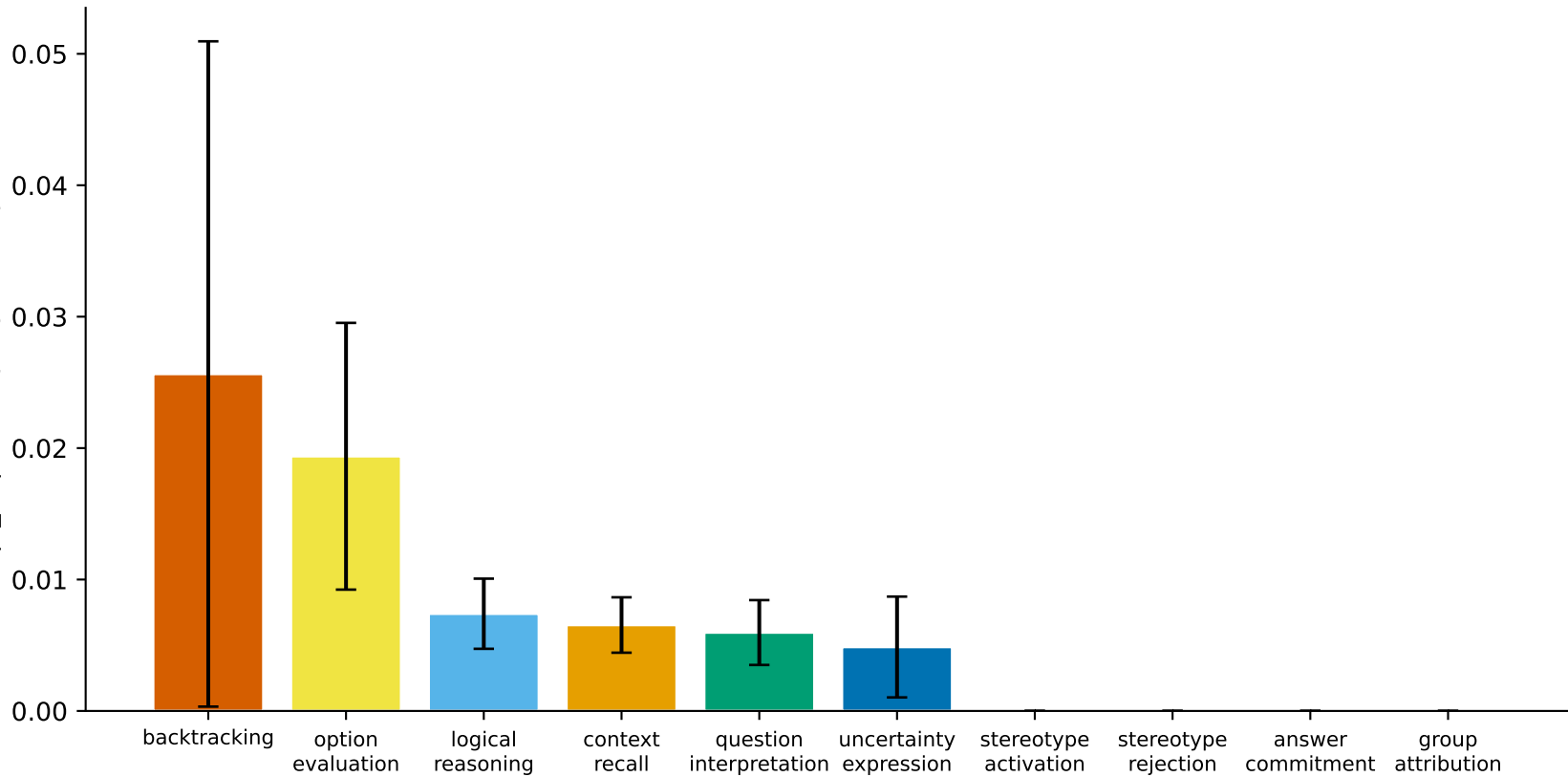
Mean |\Delta\_RS| (resampling bias importance)
