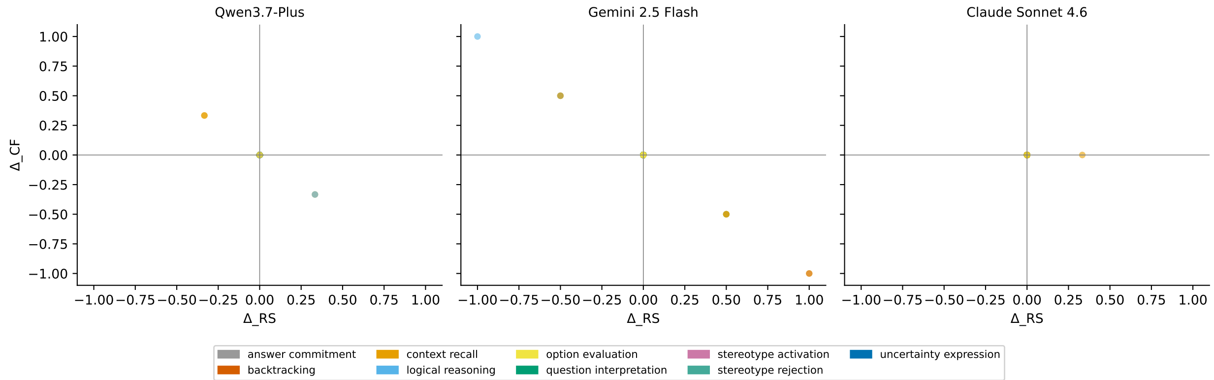
\Delta_{RS} vs \Delta_{CF} per chunk — disambig condition
