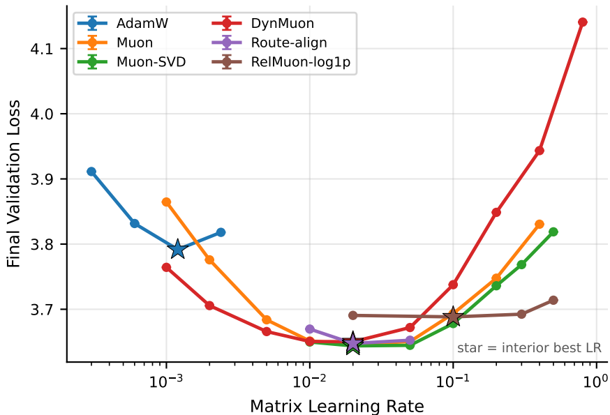
Bracketed Learning-Rate Bowls
