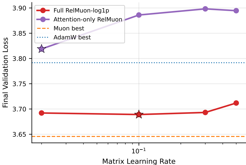
Attention-Only RelMuon Gives Up Most of the Gain
