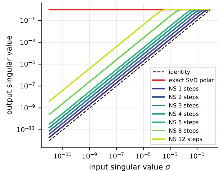
Muon Singular-Value Response
