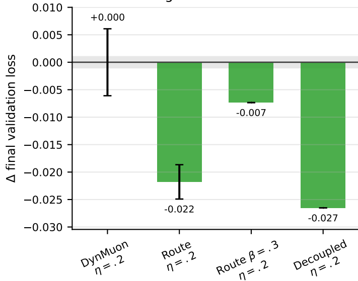
High-LR Stress Test
