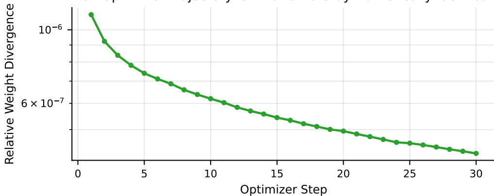
Full Optimizer Trajectory: SVD and NS Stay Numerically Identical
