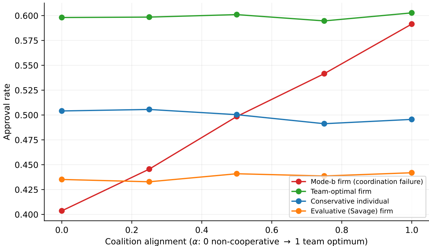
Only the mode-b firm's act responds to the alignment treatment
