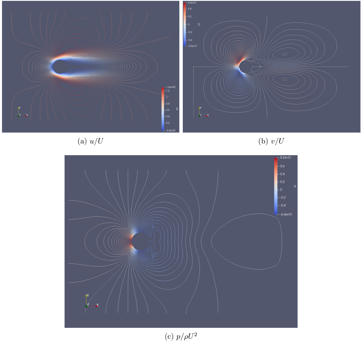
Figure 5: Velocity and pressure distributions for steady solution
