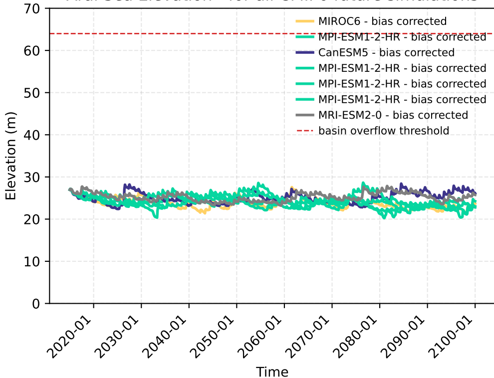
Aral Sea Elevation - for all CMIP6 future simulations
