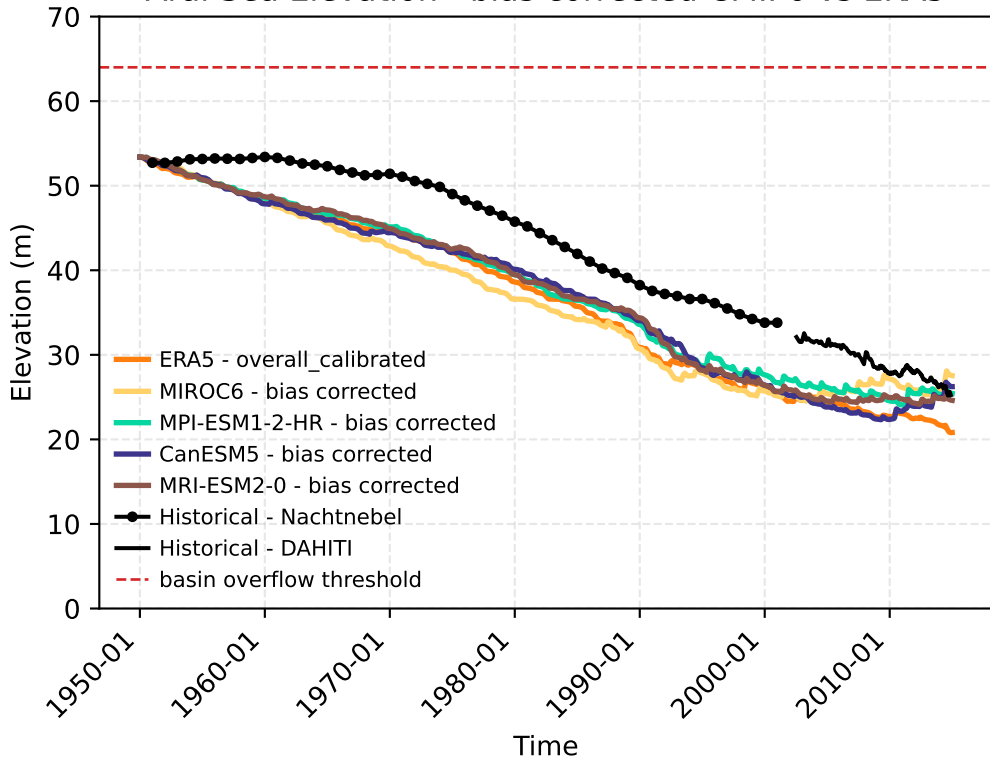
Aral Sea Elevation - bias corrected CMIP6 vs ERA5
