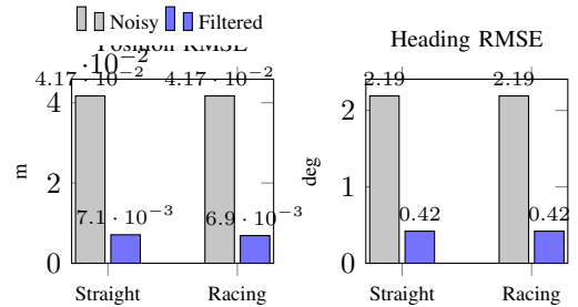
Fig. 6. Absolute RMSE values from the exported MS5 artifacts. The Kalman filter consistently reduces both position and heading error across the two evaluated scenarios.
