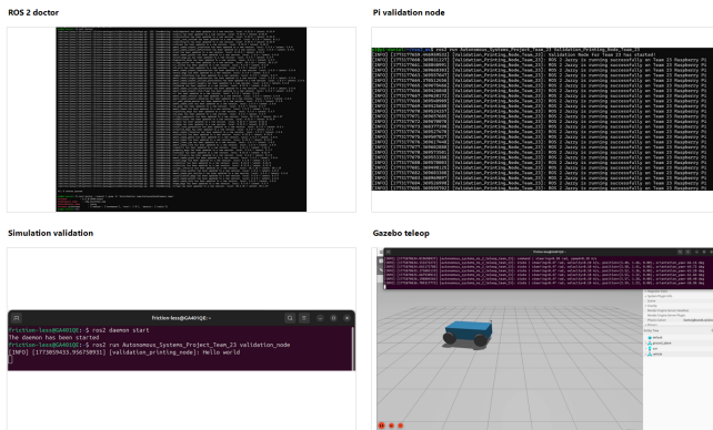
Fig. 3. Condensed bring-up evidence: ROS 2 diagnostics on the Raspberry Pi, hardware and simulation validation nodes, and Gazebo teleoperation for the initial motion and feedback path.
