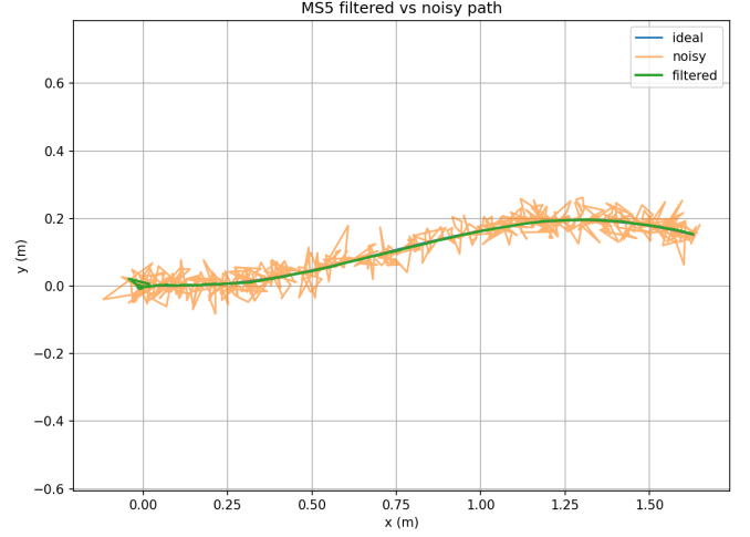
Fig. 5. Exported MS5 racing-track XY path. The filtered trajectory stays near the ideal lane-change corridor through the obstacle-avoidance sequence, while the noisy path diverges more visibly.
