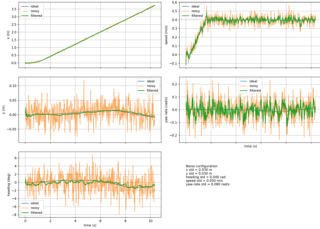
Fig. 4. Exported MS5 straight-track artifact. The filtered states follow the ideal x , y , heading, speed, and yaw-rate histories much more closely than the noisy measurements over the 10.34 s run.
