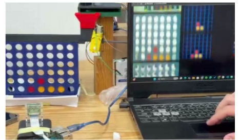
Fig. 5. System-level proof of closed-loop behavior from the final demo. A human move is accepted first, the robot plans from the trusted board, and the internal state is only advanced after the camera confirms the physical post-drop result.
