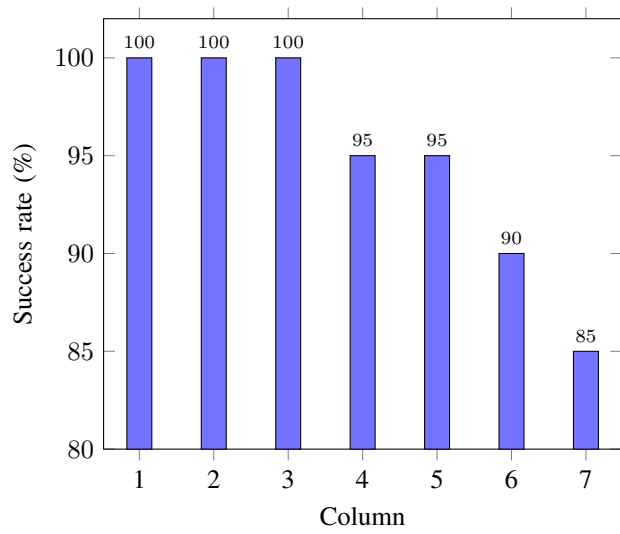
Fig. 4. Token-drop success by column. The monotonic falloff with travel distance shows that the dominant integrated failure mode is carriage positioning at the board edges, not token recognition.
