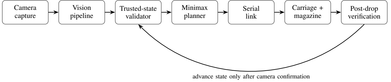
Fig. 1. Integrated closed-loop architecture. The camera is used twice: first to infer a candidate board and later to confirm that the physical robot move actually happened. This is the core difference between a working pipeline demo and a trustworthy integrated robot.
