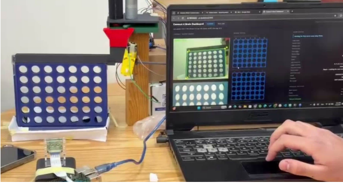
Fig. 2. Final assembled evaluation setup. The physical board, overhead dispenser, camera mount, Raspberry Pi, and operator dashboard are visible in one frame, showing the exact integrated system used in the final demonstrations.
