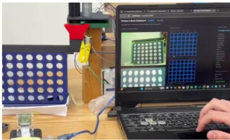
Fig. 5. System-level proof of closed-loop behavior from the final demo. A human move is accepted first, the robot plans from the trusted board, and the internal state is only advanced after the camera confirms the physical post-drop result.
