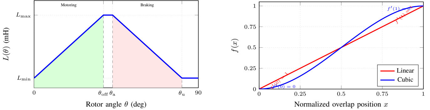
Fig. 3. Theory figure with direct physical payoff. Left: the 6/4 SRM produces positive torque only in the rising-inductance interval. Right: the selected cubic torque sharing law f(x) = 3x^2 - 2x^3 has zero slope at both overlap boundaries, unlike the linear law, so the current reference enters and exits commutation smoothly instead of with a step.
