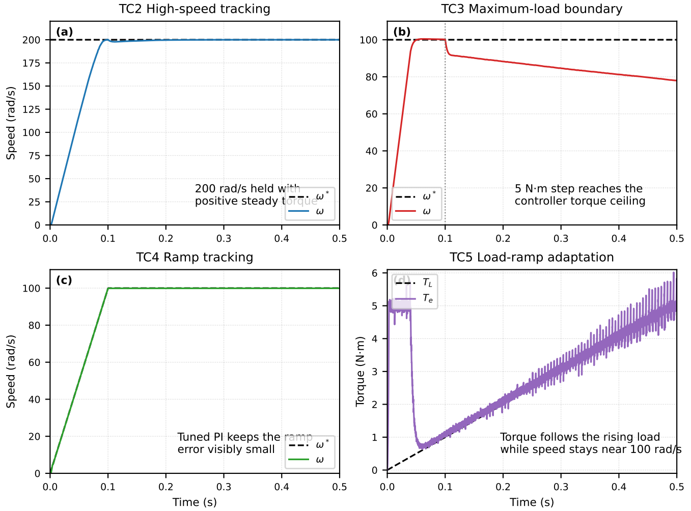
Fig. 5. Operating-envelope composite derived from TC2–TC5. (a) TC2 confirms high-speed tracking at 200 rad/s. (b) TC3 shows the saturation boundary under the maximum 5 N·m step load. (c) TC4 demonstrates low-error ramp tracking after retuning the outer loop. (d) TC5 shows torque following a continuous load ramp while speed stays close to the 100 rad/s target.
