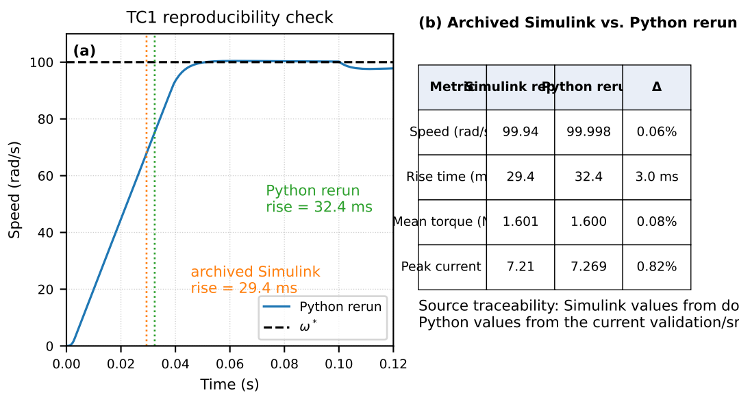
Fig. 6. Independent TC1 reproducibility check. The left panel shows the rerun Python speed trace with the archived Simulink and current Python rise-time markers. The right panel compares archived Simulink metrics from docs/Validation_Report.pdf against the current Python rerun from validation/srm_validation.py.
