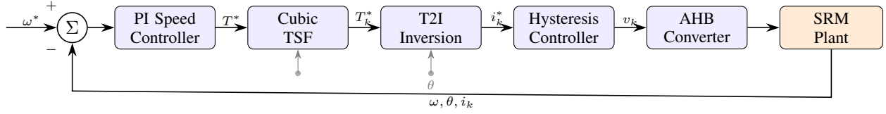
Fig. 2. Full cascaded drive architecture implemented in the project. The outer PI loop generates total torque demand, the cubic TSF allocates phase torques, the T2I block maps them to current references, the hysteresis loop switches the asymmetric half-bridge, and the SRM plant feeds back speed, angle, and currents.
