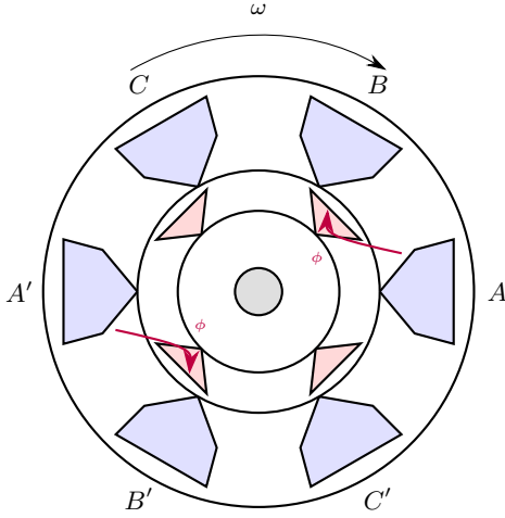
Fig. 1. 6/4 SRM cross-section with three stator phases and four rotor poles. Opposite stator teeth form one phase pair, while torque is produced as the rotor moves toward the energized low-reluctance path.
