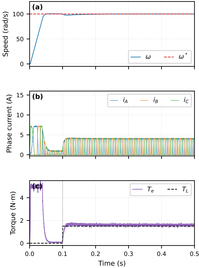
Fig. 4. Representative baseline response for TC1. The speed loop reaches the 100 rad/s command, the cubic TSF shapes the three phase currents through commutation, and the electromagnetic torque settles to the 1.5 N m load after startup saturation clears.
