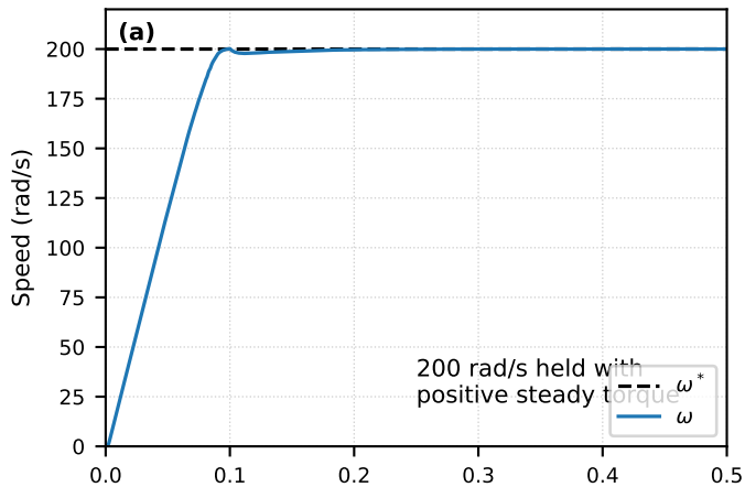
TC4 Ramp tracking
