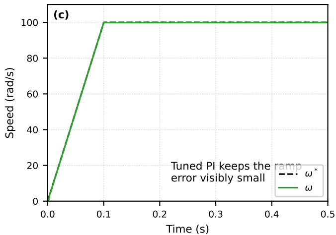
TC4 Ramp tracking
