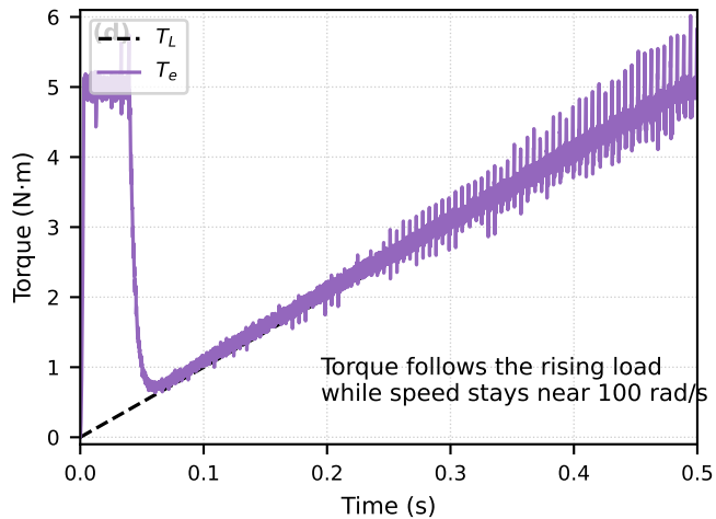
TC5 Load-ramp adaptation
