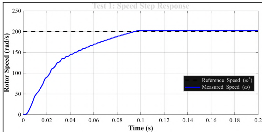
(a) Rotor Speed Response (200 rad/s)
