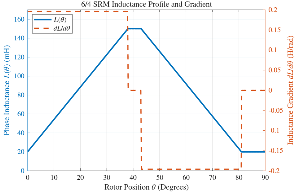
Figure 2.1: Idealized piecewise-linear inductance profile L(\theta) and its corresponding gradient dL/d\theta for a single phase of the 6/4 SRM over one complete rotor pole pitch ( 90^\circ ).
