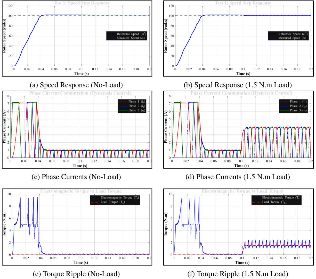
Figure 4.1: TC1: Performance characteristics of the 6/4 SRM illustrating the synchronization between mechanical velocity, programmatic phase excitation, and total electromagnetic torque under baseline conditions.
