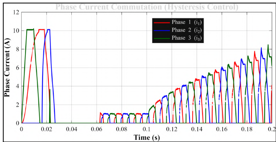
(b) Phase Currents (Load-Dependent Scaling)
