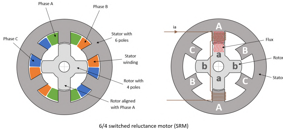
Figure 1.1: Cross-section and Flux Distribution of a 6/4 Switched Reluctance Motor. The left illustration shows the concentrated windings of the three phases, while the right depicts the flux path and rotor alignment in the low-reluctance position during Phase A excitation [1].
