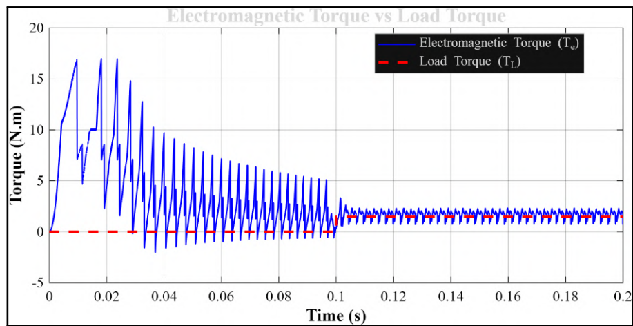
(c) Electromagnetic Torque
