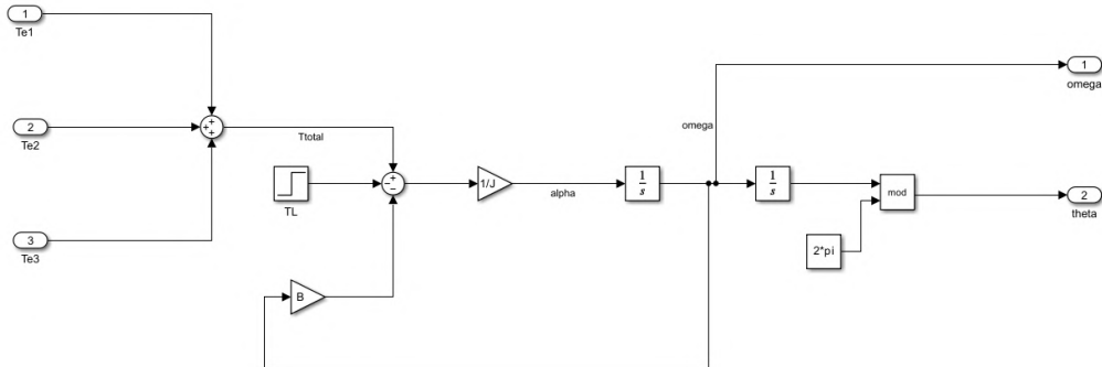
Figure 3.2: Simulink implementation of the Mechanical Dynamics subsystem. The model aggregates the three individual phase torques and subtracts the external load torque ( T_L ) and viscous friction ( B\omega ). The resulting net torque is processed through an inertial gain ( 1/J ) and integrated to determine the rotor speed ( \omega ) and mechanical position ( \theta ).
