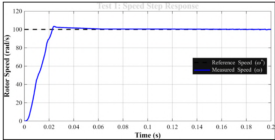
(a) Rotor Speed (Steady-State Accuracy)
