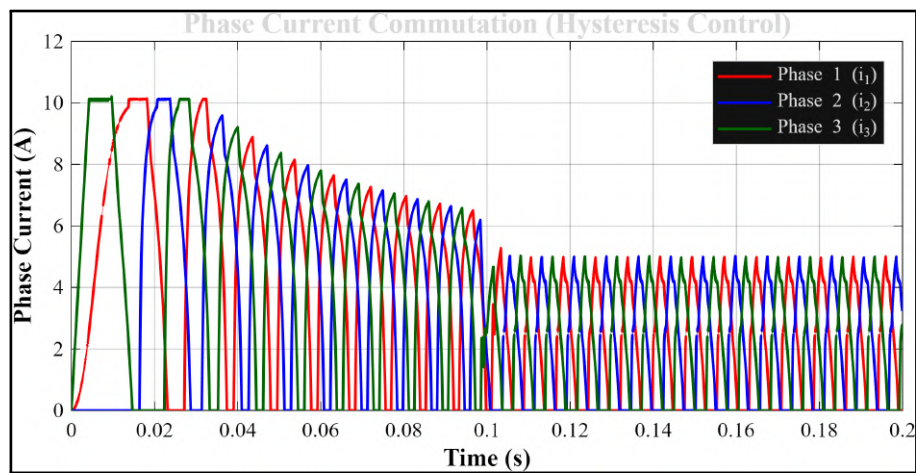
(b) Phase Currents (Increased Back-EMF influence)
