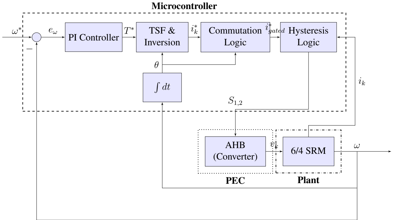
Figure 3.3: Cascaded control architecture distinguishing the software microcontroller logic, the physical power converter, and the motor plant.
