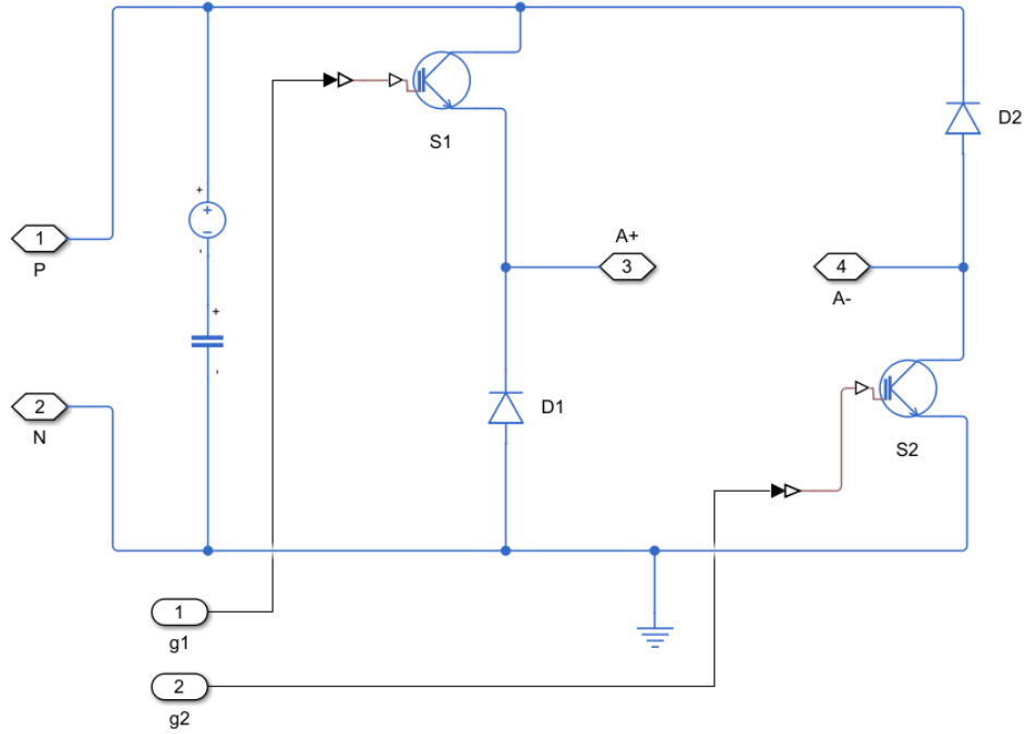
Figure 2.2: Schematic of an Asymmetric Half-Bridge (AHB) implemented in Simscape/Simulink for a single SRM phase, illustrating the diagonal arrangement of the two active switches ( S_1 , S_2 ) and two freewheeling diodes ( D_1 , D_2 ) around the phase winding represented by the ports A+ and A-.
