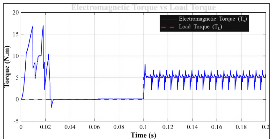
(c) Electromagnetic Torque (5.0 N.m Balance)
