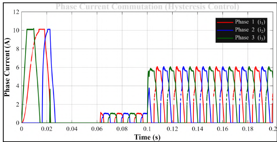
(b) Phase Currents (High-Magnitude Regulation)
