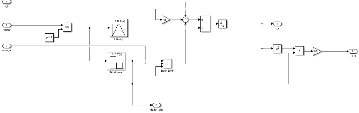
Figure 3.1: Simulink implementation of the 6/4 SRM Phase Dynamics subsystem. The model realizes the electrical state equation by integrating the derivative of current ( di/dt ), calculated as the net voltage (source minus resistive drop and back-EMF) divided by the instantaneous inductance L(\theta) provided by the 1-D Look-Up Table. The lower branch implements the quadratic torque production logic: T_e = \frac{1}{2} i^2 \frac{dL}{d\theta} .
