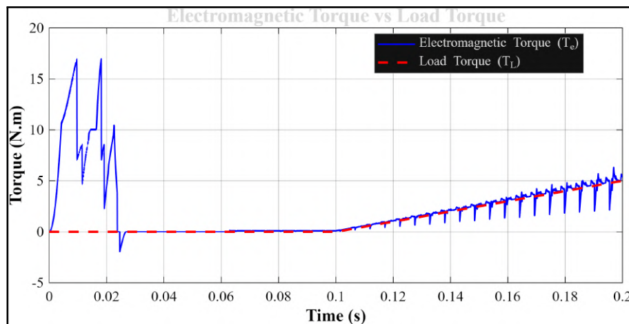
(c) Electromagnetic Torque (Ramp Disturbance Rejection)
