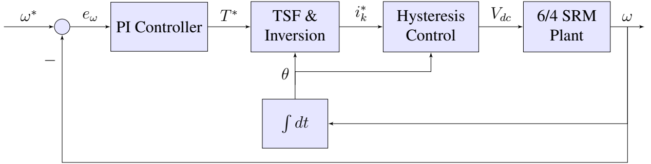
Figure 3.3: Cascaded control architecture for the 6/4 SRM featuring outer-loop speed regulation and inner-loop current control. The diagram illustrates the integration of speed and position feedback through a Torque Sharing Function (TSF) and hysteresis regulators to manage the non-linear motor dynamics.
