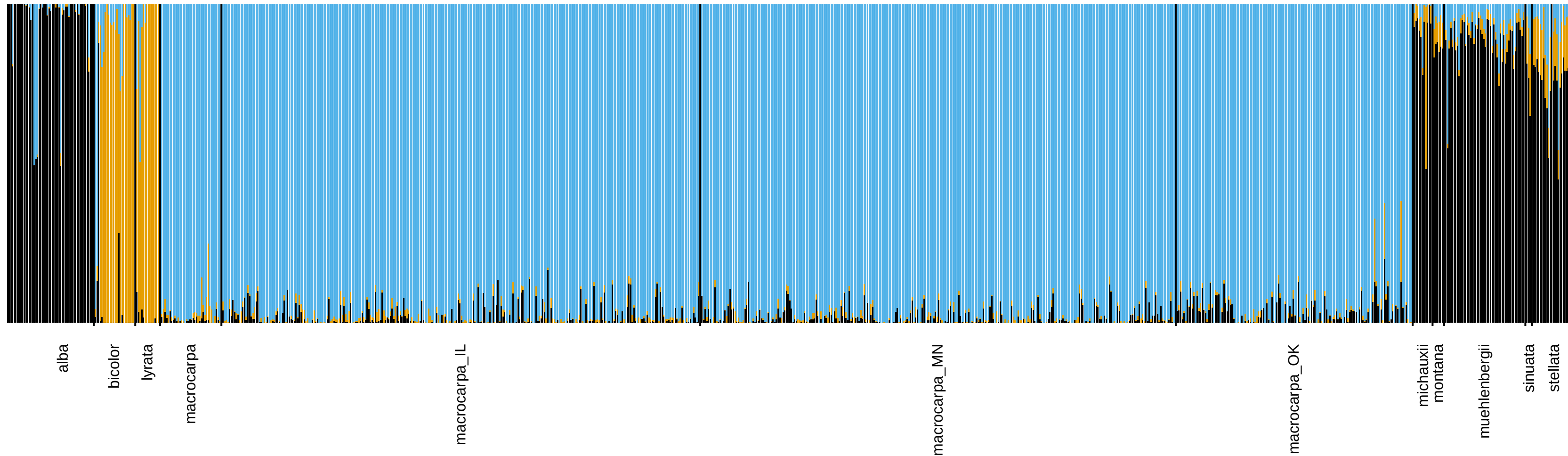
MOR ACE experiment, K = 4_viz_3
