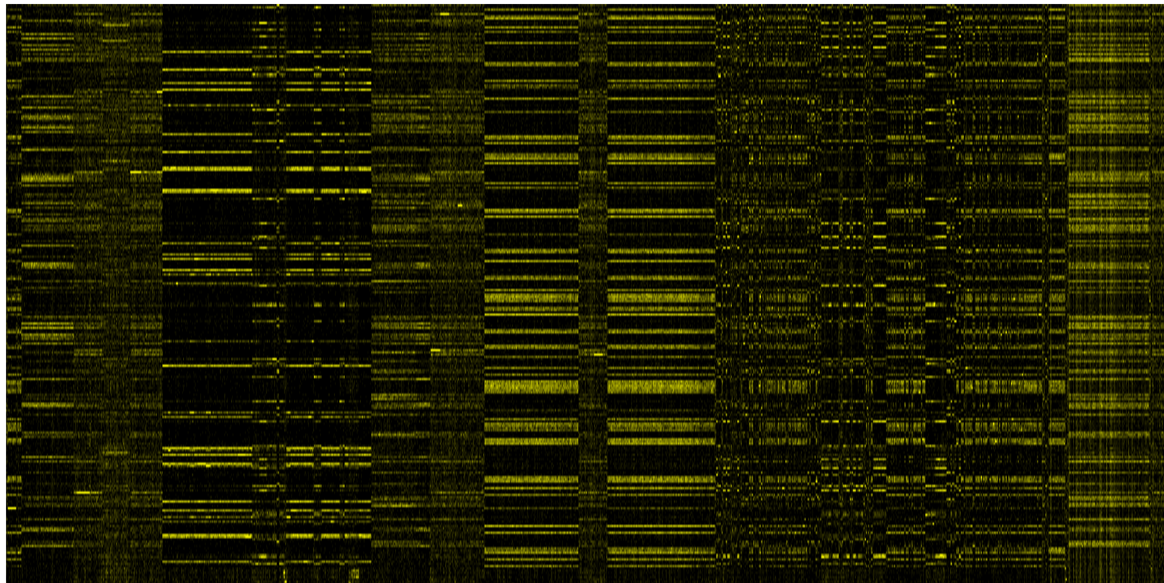
Oak supermatrix: data present (yellow) vs. missing (black) | 261 taxa x 1,969,938 sites
