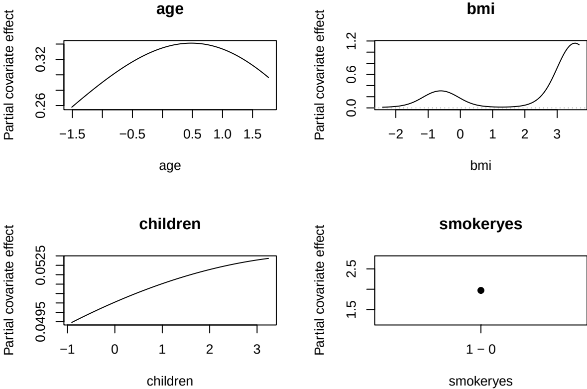
Figure 4: Partial covariate-effect plots for selected covariates in the insurance data. The panels show estimated covariate effects for age, body mass index, number of children, and smoking status.
