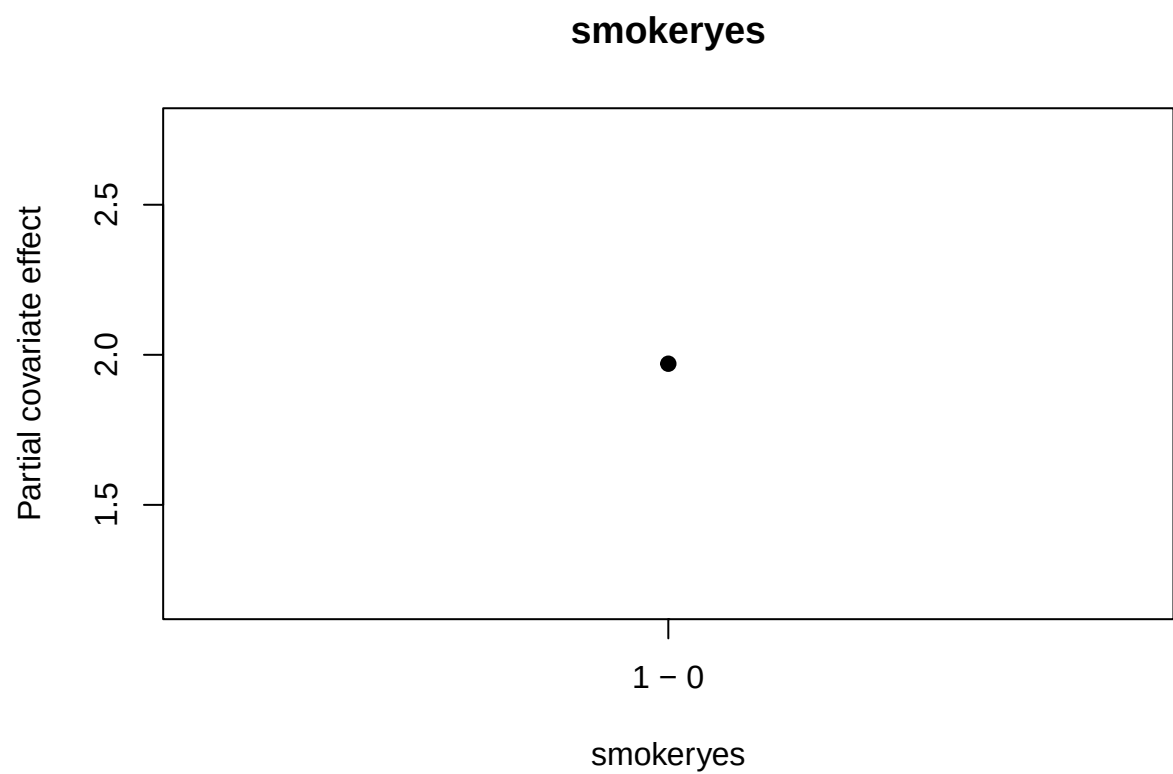
Figure 3: Partial covariate-effect plot for smoking status in the insurance data. The plot shows the estimated change in fitted charges associated with the smoking-status dummy variable.
