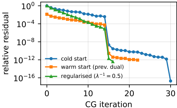
Krylov control projection: CG convergence
