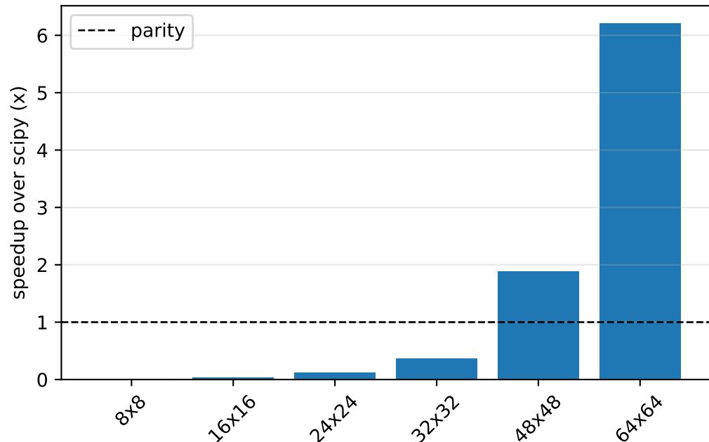
Histogram vs exact KDE (below parity = histogram is slower)
