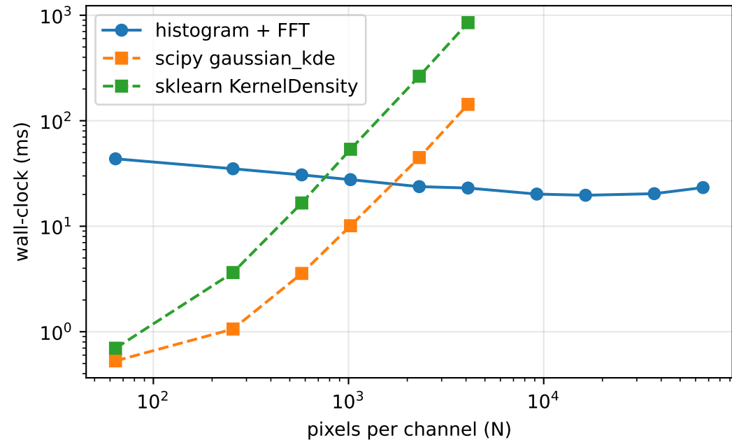
Log-density estimation cost
