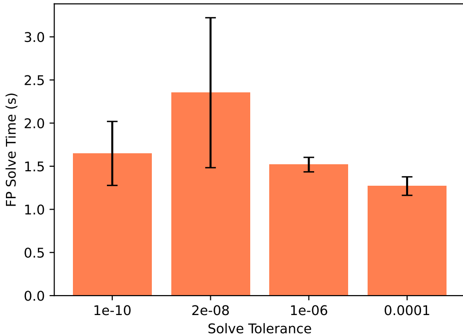
FP Time vs Solve Tolerance
