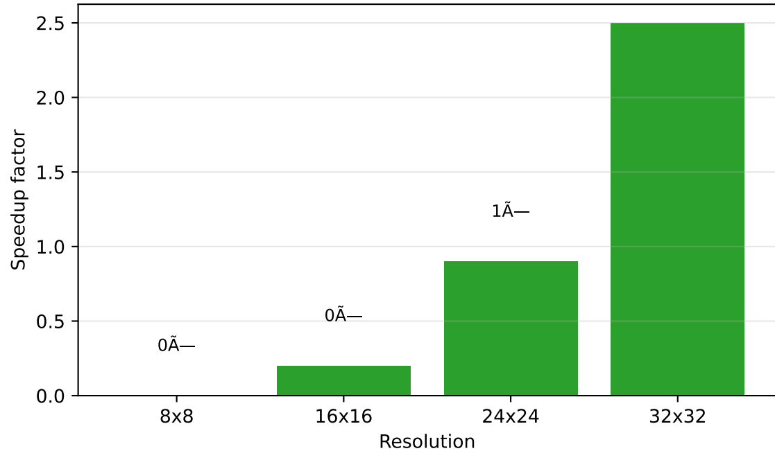
Speedup: Histogram FFT over scipy KDE 2^{\frac{N}{2}}
