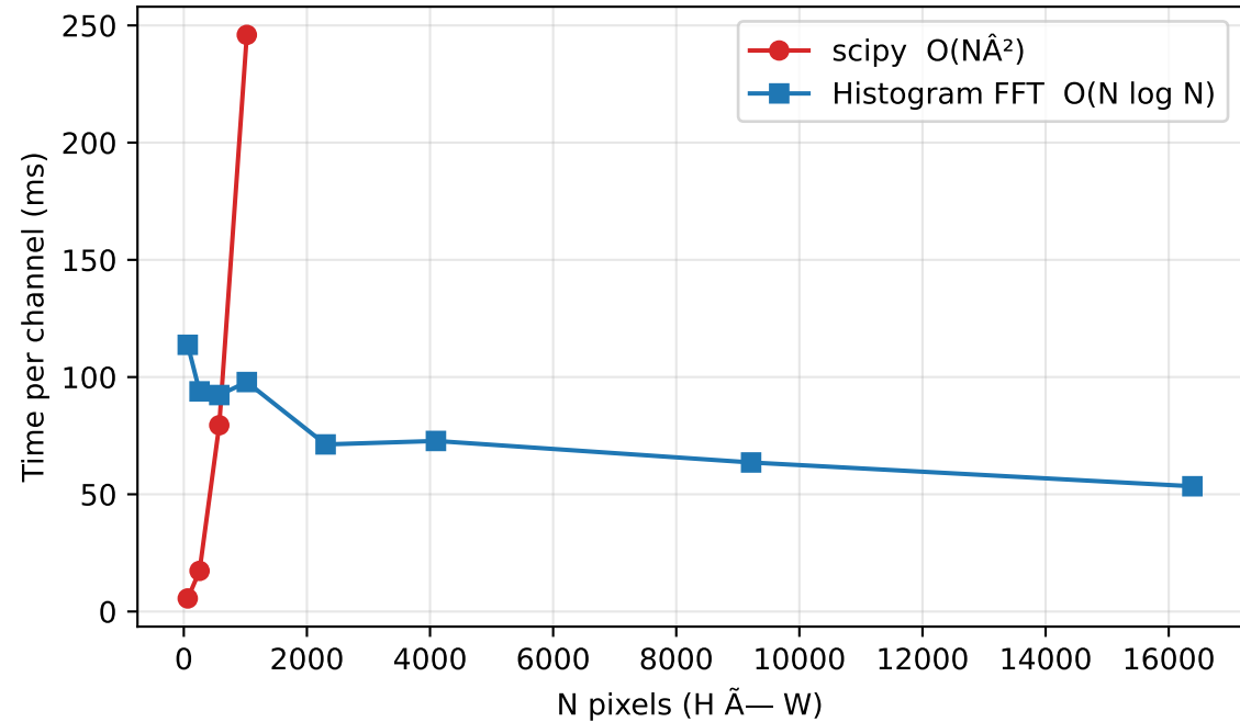
KDE Timing vs Image Size
