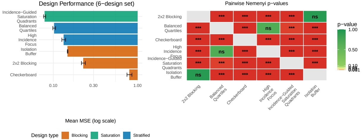
Figure S5: Left: mean MSE per design (log scale, \tau = 1.0 ) with \pm 1 standard error bars, colored by conceptual design group (Blocking: Checkerboard, 2×2 Blocking, Isolation Buffer; Stratified: High Incidence Focus, Balanced Quartiles; Saturation: Incidence-Guided Saturation Quadrants). Right: pairwise Nemenyi p -value heatmap for the six retained designs; dark red cells are statistically significant ( p < 0.05 ).
