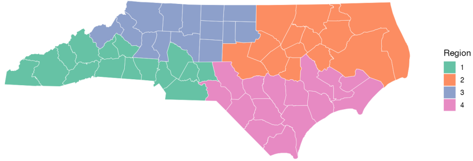
Figure S14: Frozen four-region partition used by both saturation strategies in all years, chosen from 250 geographic candidates before outcome evaluation.
