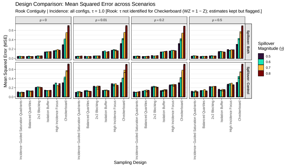
Figure S11: Mean squared error of the oracle estimate of \tau by design at \tau = 1 , under rook contiguity; layout as in Figure S2. Checkerboard is flagged ( \tau not identified).
