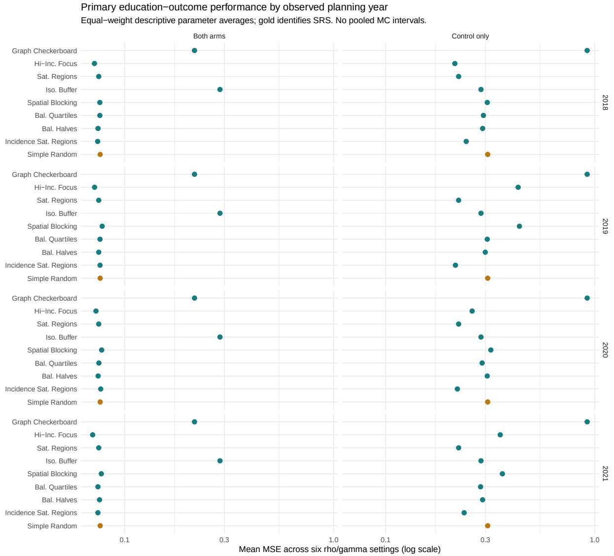
Figure S18: Completed primary application: mean MSE by design, planning year and spillover regime, queen contiguity and education outcome. Each entry equally averages the six \rho/\gamma pairs. Both regime columns use a common logarithmic MSE scale. Shared annual sources are repeated reporting, not independent replications; pooled Monte Carlo intervals are not supplied.
