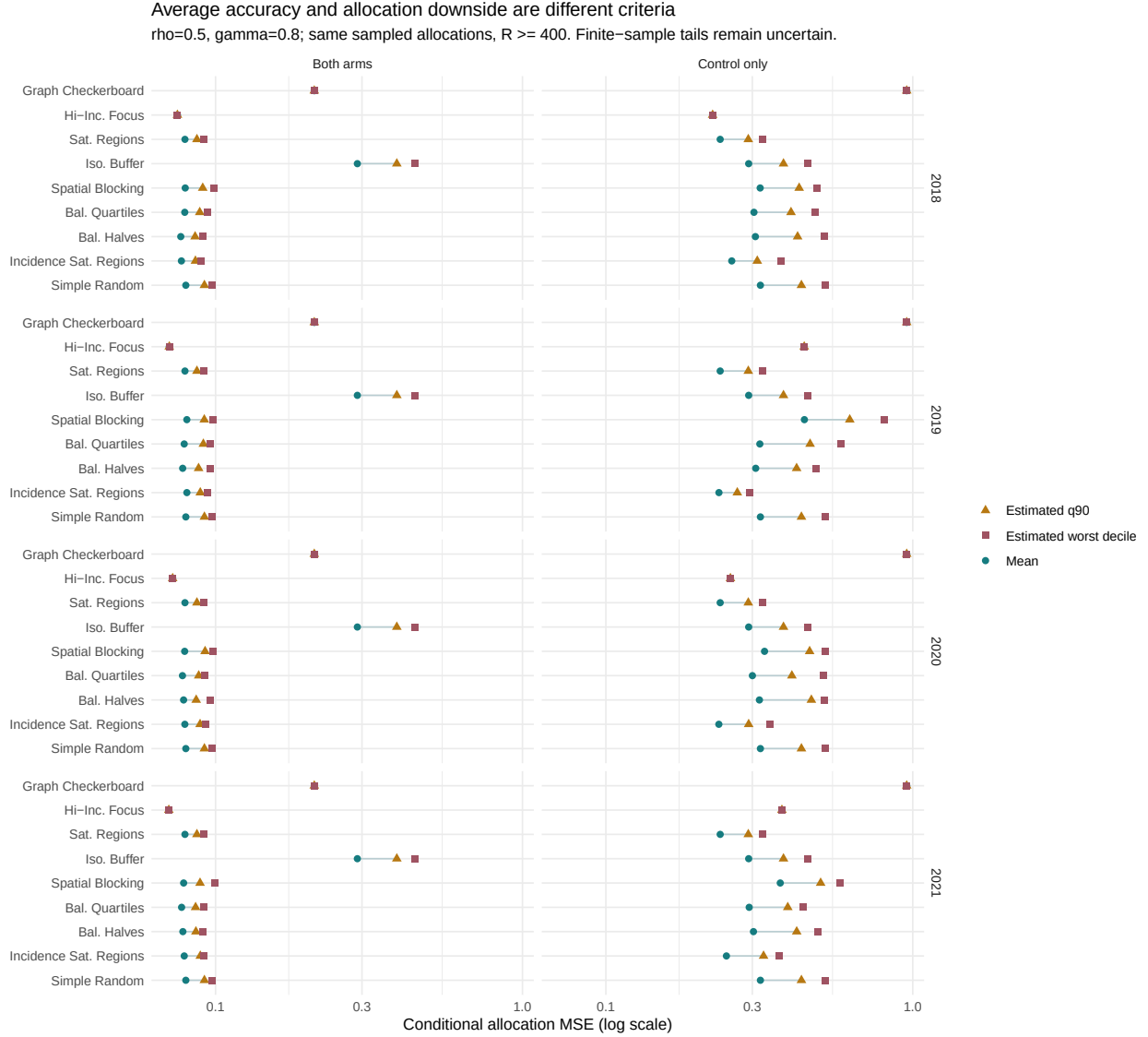
Figure S19: Allocation-specific conditional MSE in the refined primary queen setting \rho = 0.5 , \gamma = 0.8 , by year and spillover regime. Mean MSE, estimated allocation q90 and estimated worst-decile mean summarize the same J = 100 sampled assignments, with at least 400 independent outcomes per stochastic assignment or 1,000 for singleton supports. These finite-outcome tail estimates are descriptive, with uncertain membership; they are not quantiles of realized errors or a fresh allocation confirmation.
