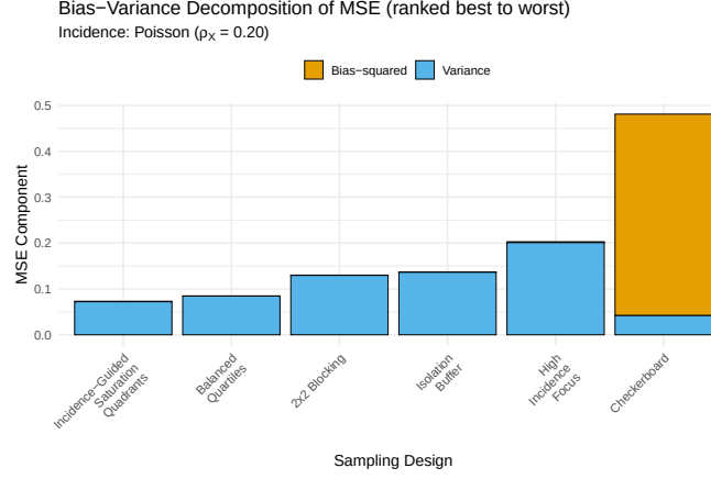
Figure 13: Squared bias and variance of \hat{\tau} by design at \tau = 1 for the Poisson configuration with \rho_X = 0.20 , under rook contiguity; layout as in Figure 4. Checkerboard is flagged ( \tau not identified).
