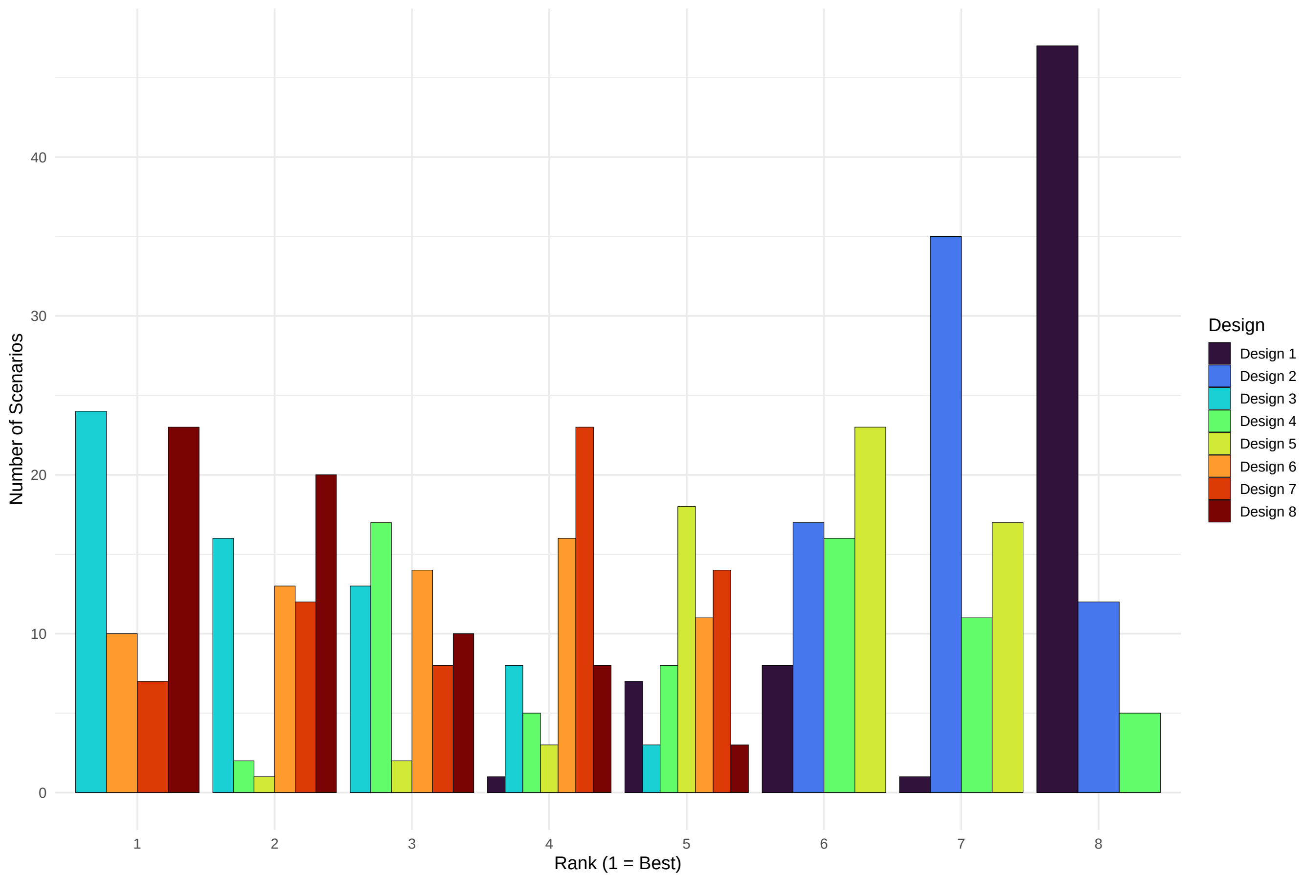
Design Rank Distribution across Scenarios Incidence: Spatial ( \rho_X = 0.20 ) | Rank 1 = lowest MSE in that scenario
