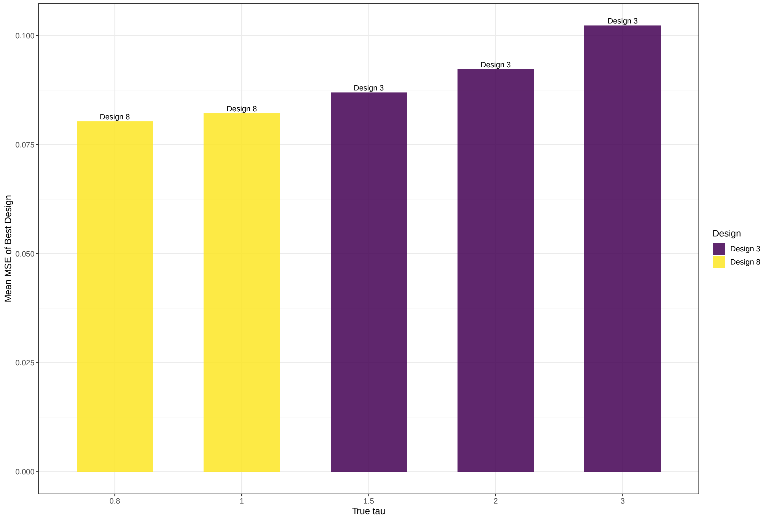
Best Design (Lowest MSE) at Each Tau Value Spatial ( \rho_X = 0.50 )
