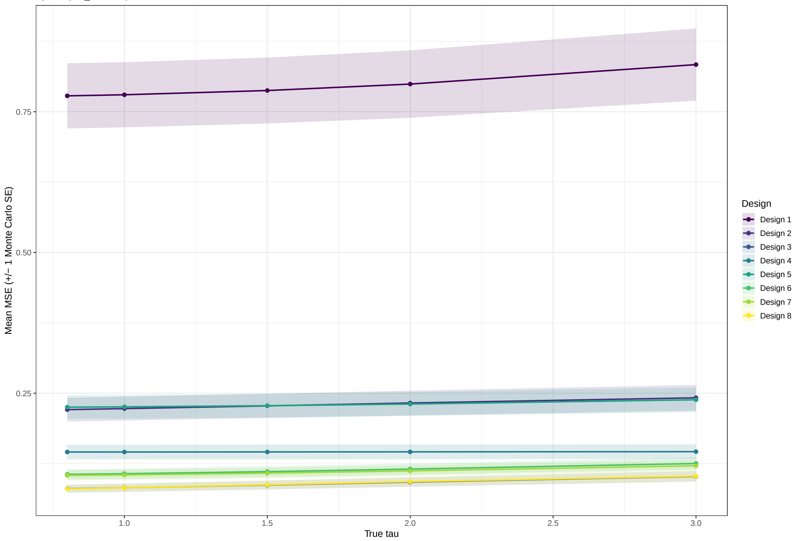
MSE vs. True Tau by Design Spatial ( \rho_X = 0.50 )
