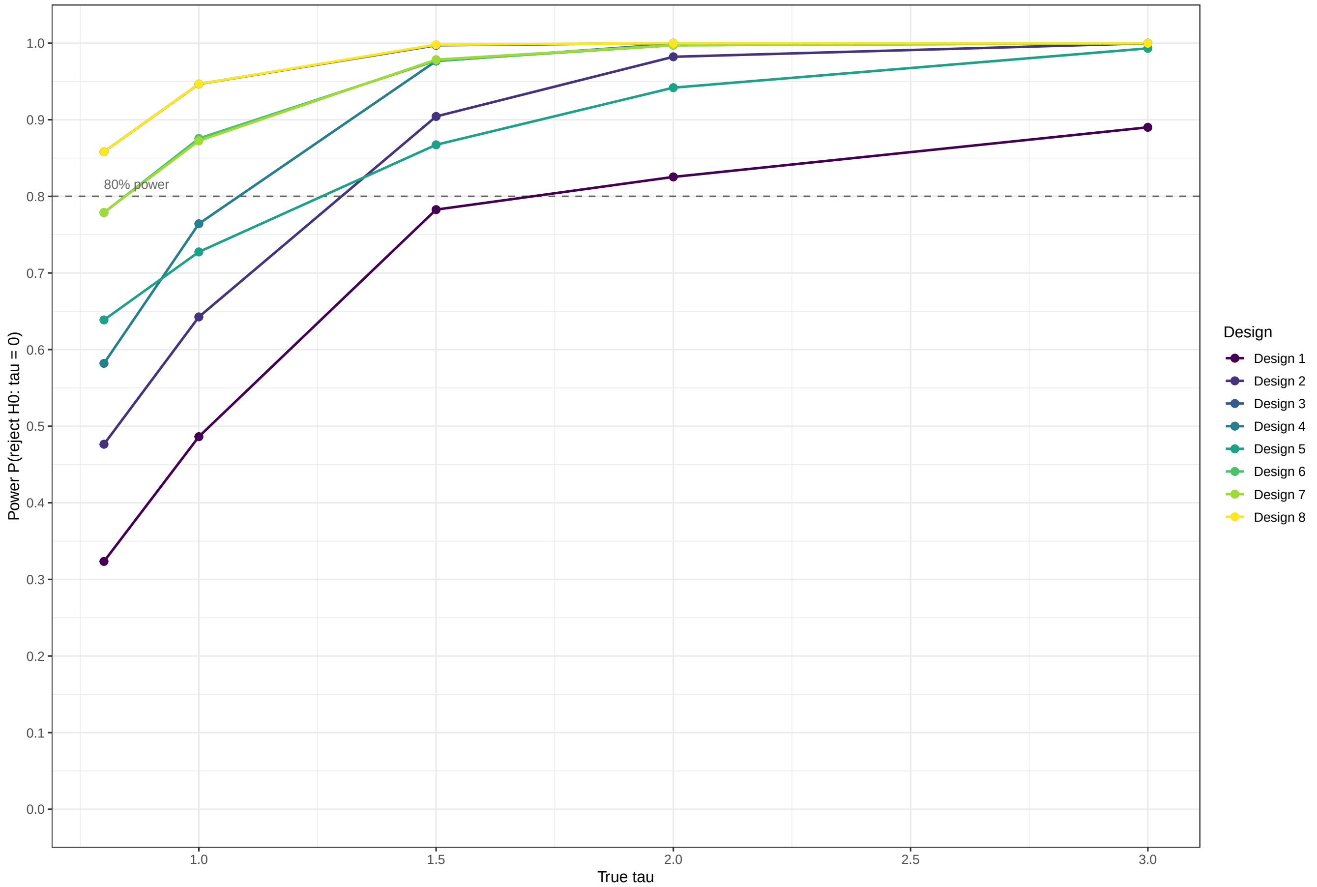
Statistical Power by Design Across Tau Values Spatial ( \rho_X = 0.50 )
