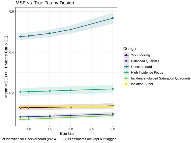
(b) Rook contiguity (sensitivity)
