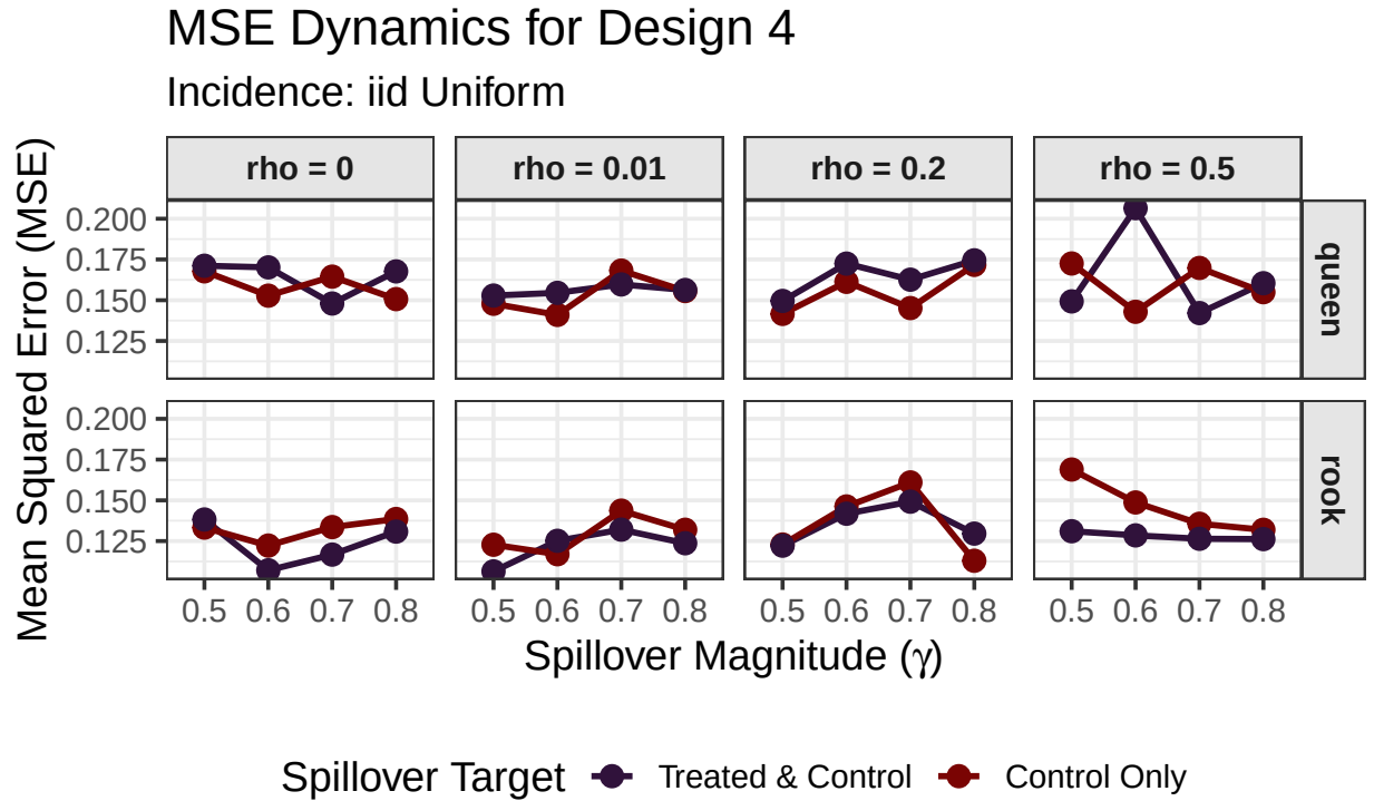
Figure 21: Per-design MSE line plots across gamma levels, for iid Uniform incidence ( \tau = 1.0 ).
