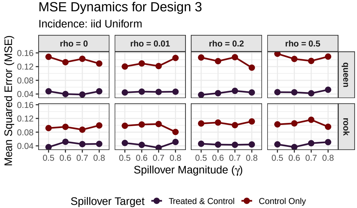
Figure 20: Per-design MSE line plots across gamma levels, for iid Uniform incidence ( \tau = 1.0 ).
