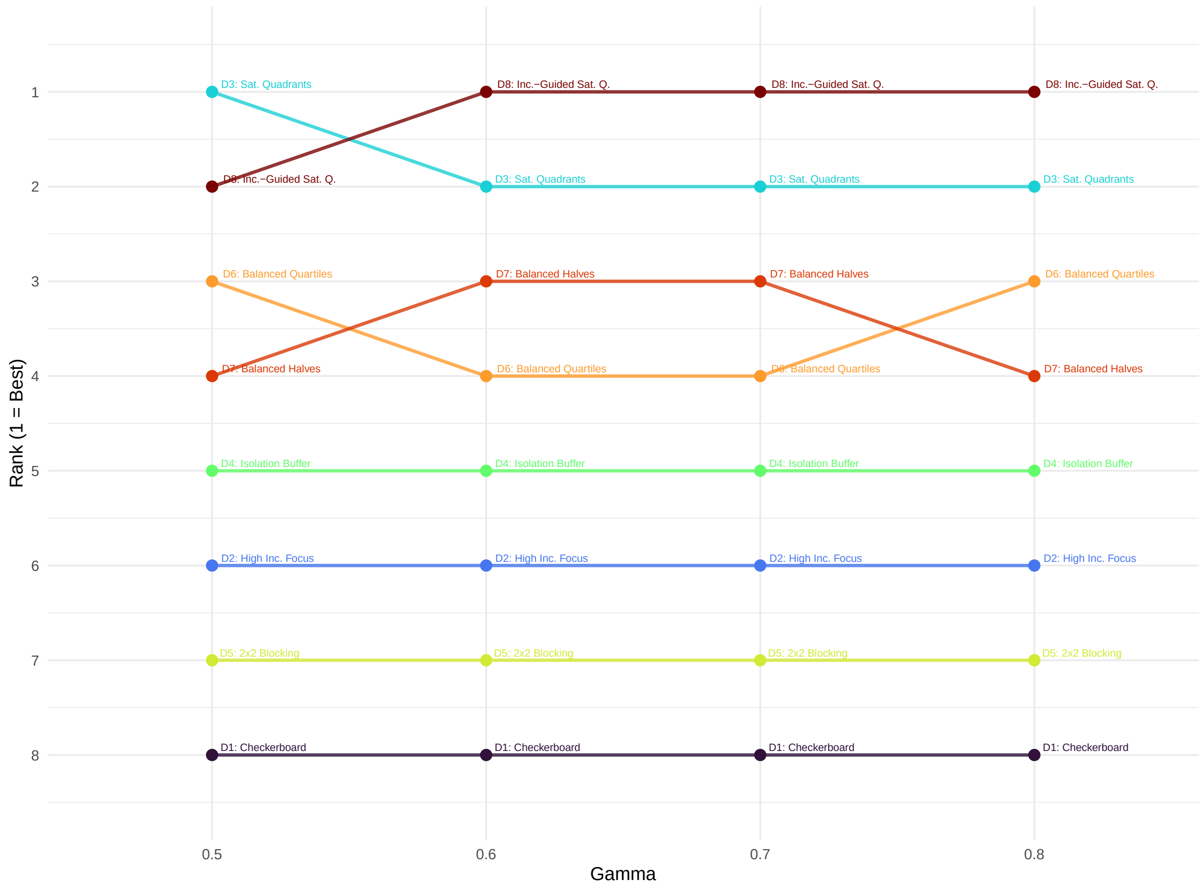
Design Rank Trajectories across Gamma Incidence: Spatial ( \rho_X = 0.20 ) | Rank 1 = lowest avg MSE
