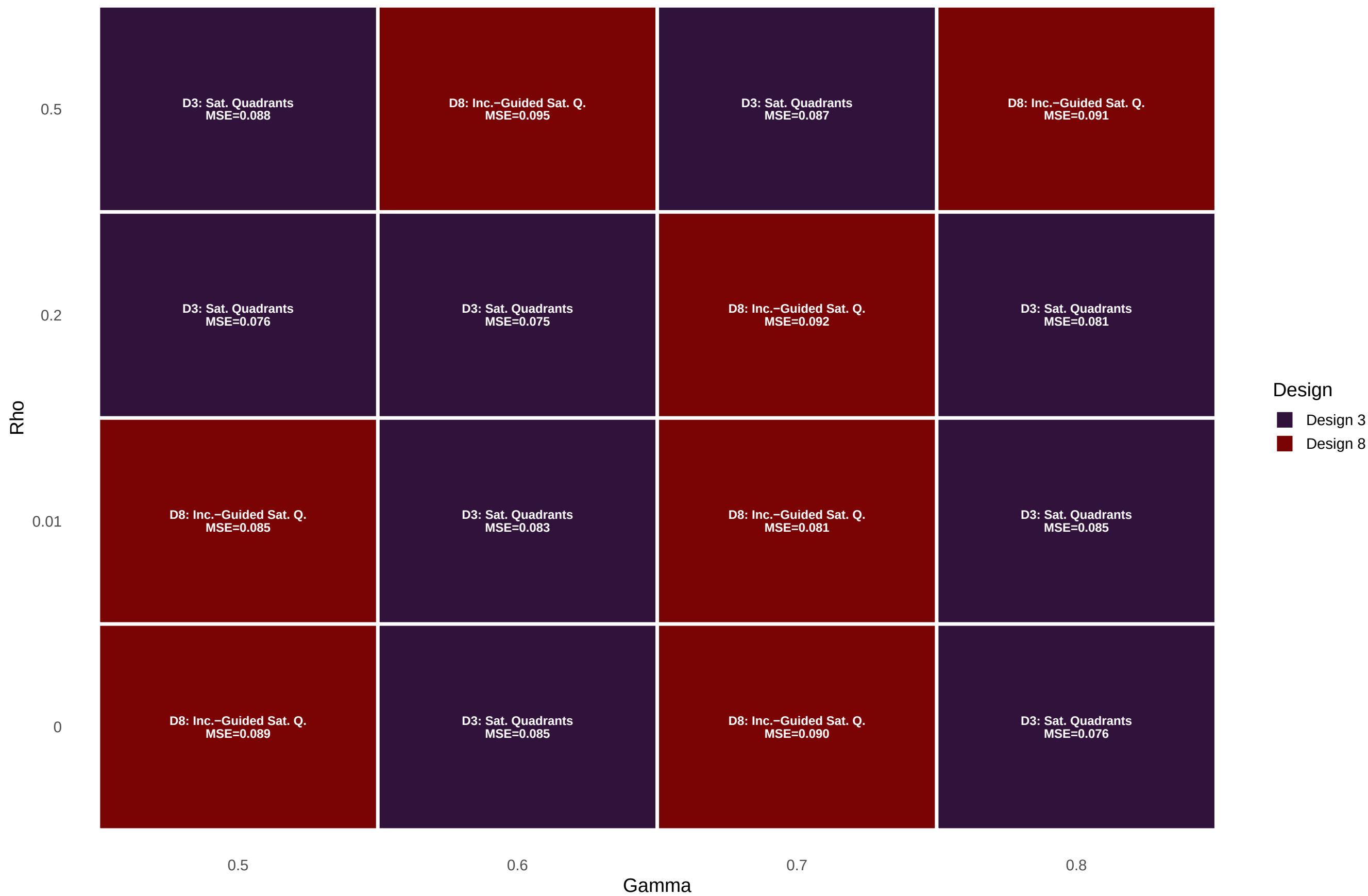
Best Design by Rho x Gamma Incidence: Poisson (rho_X = 0.20) | Cell = best design (lowest avg MSE across other params)
