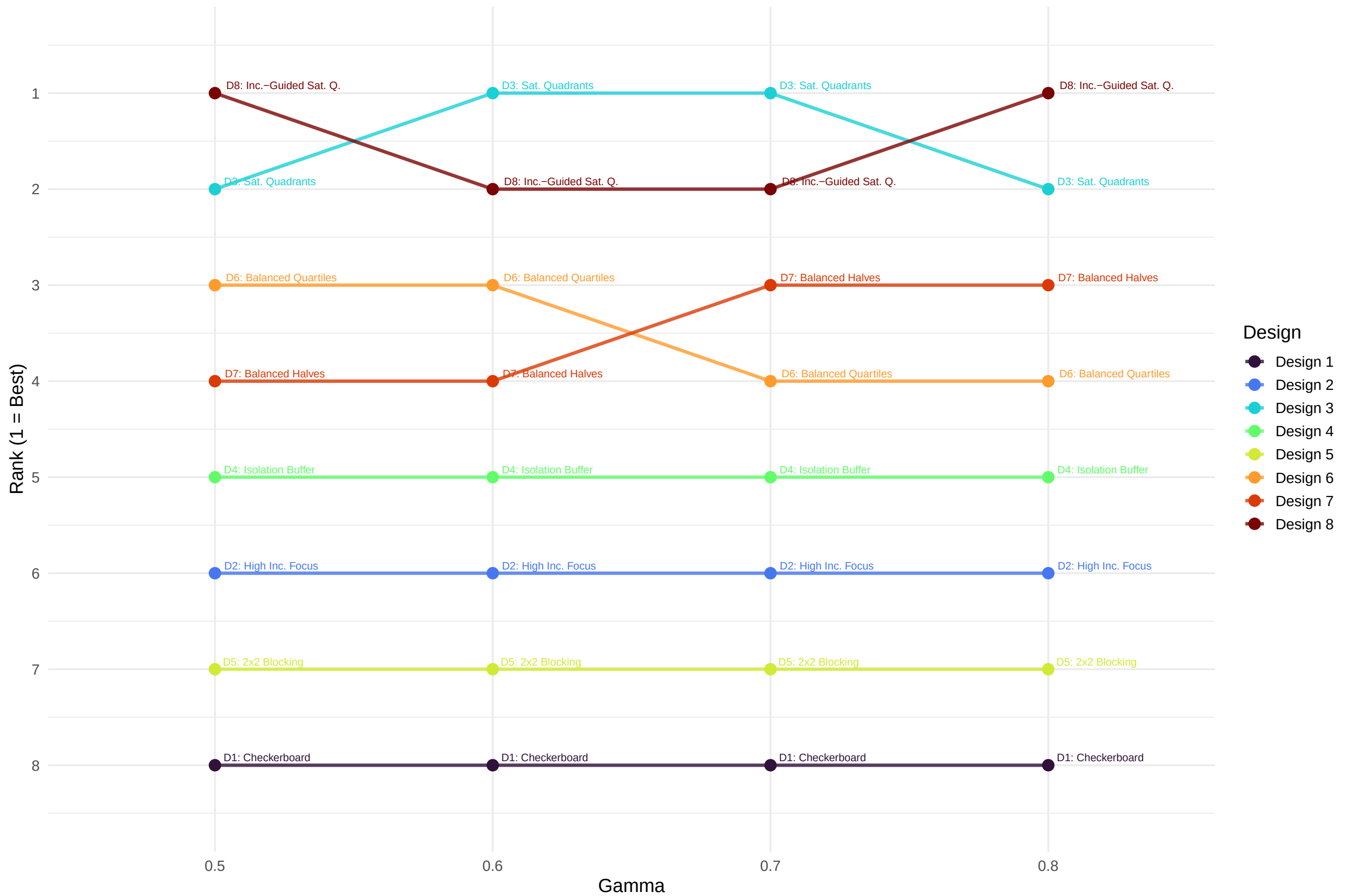
Design Rank Trajectories across Gamma Incidence: iid Uniform | Rank 1 = lowest avg MSE
