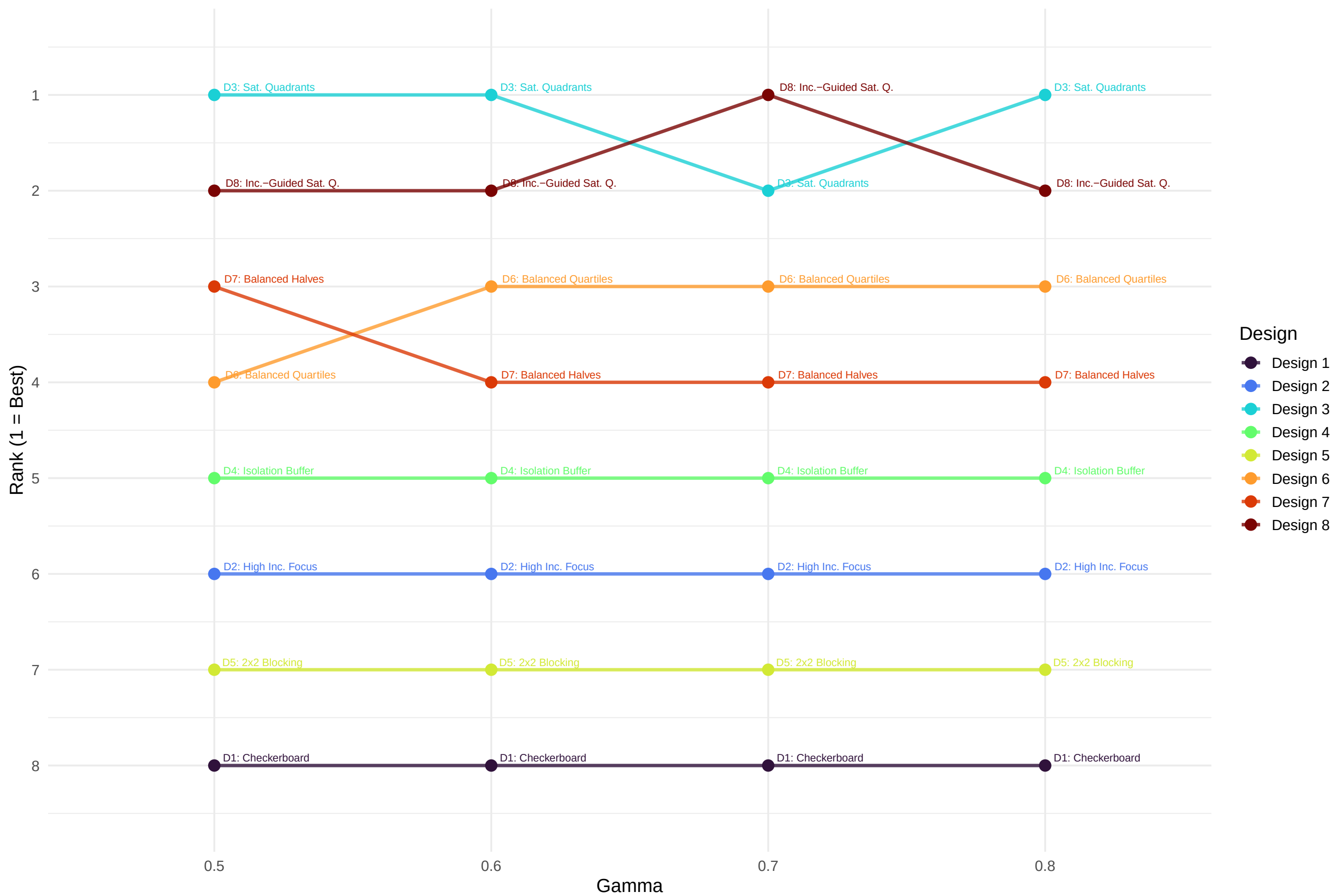
Design Rank Trajectories across Gamma Incidence: Poisson ( \rho_X = 0.20 ) | Rank 1 = lowest avg MSE
