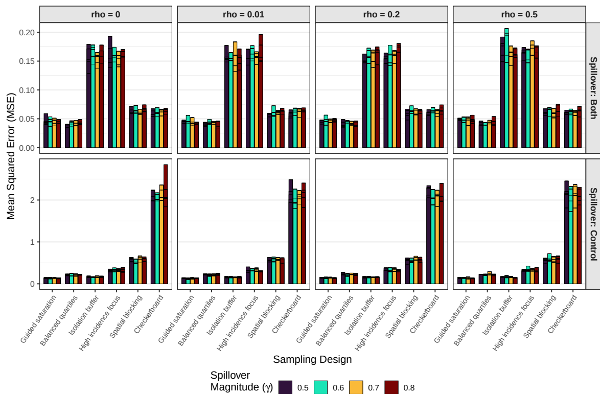
Figure 1. Grid MSE at \tau = 1 under queen contiguity for the detailed six-design subset. Columns show outcome spatial dependence and rows spillover regimes. Bars overlay five incidence configurations, with horizontal lines marking their values; colors show spillover magnitude. Table 1 additionally includes plain saturation, Balanced Halves and SRS. Regime scales differ.
