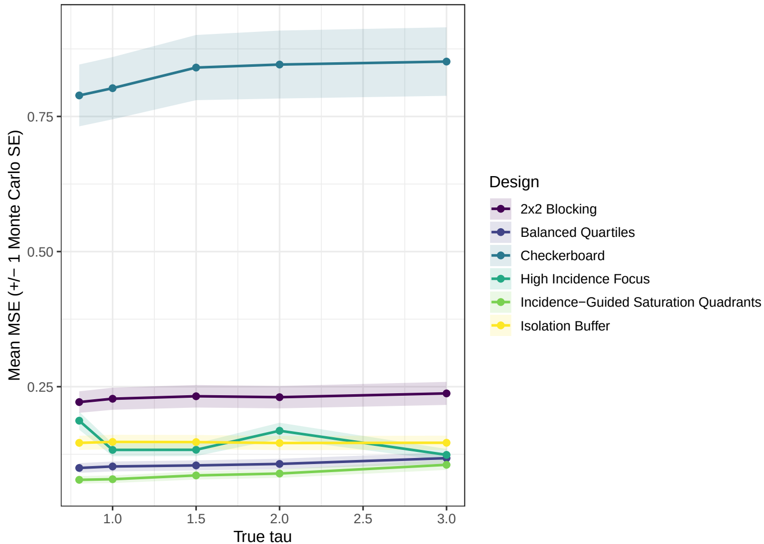
MSE vs. True Tau by Design
